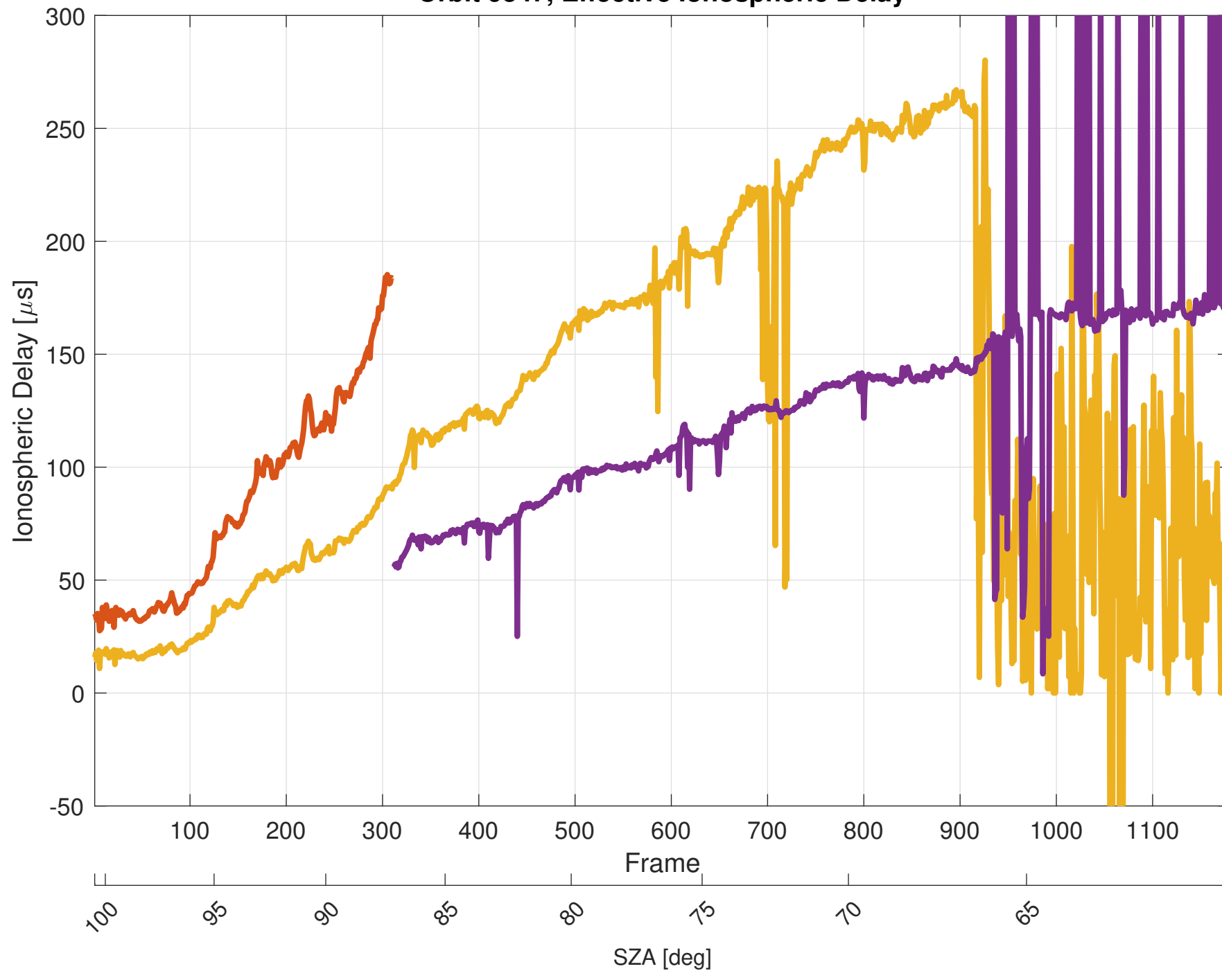
Orbit 9347, Effective Ionospheric Delay
