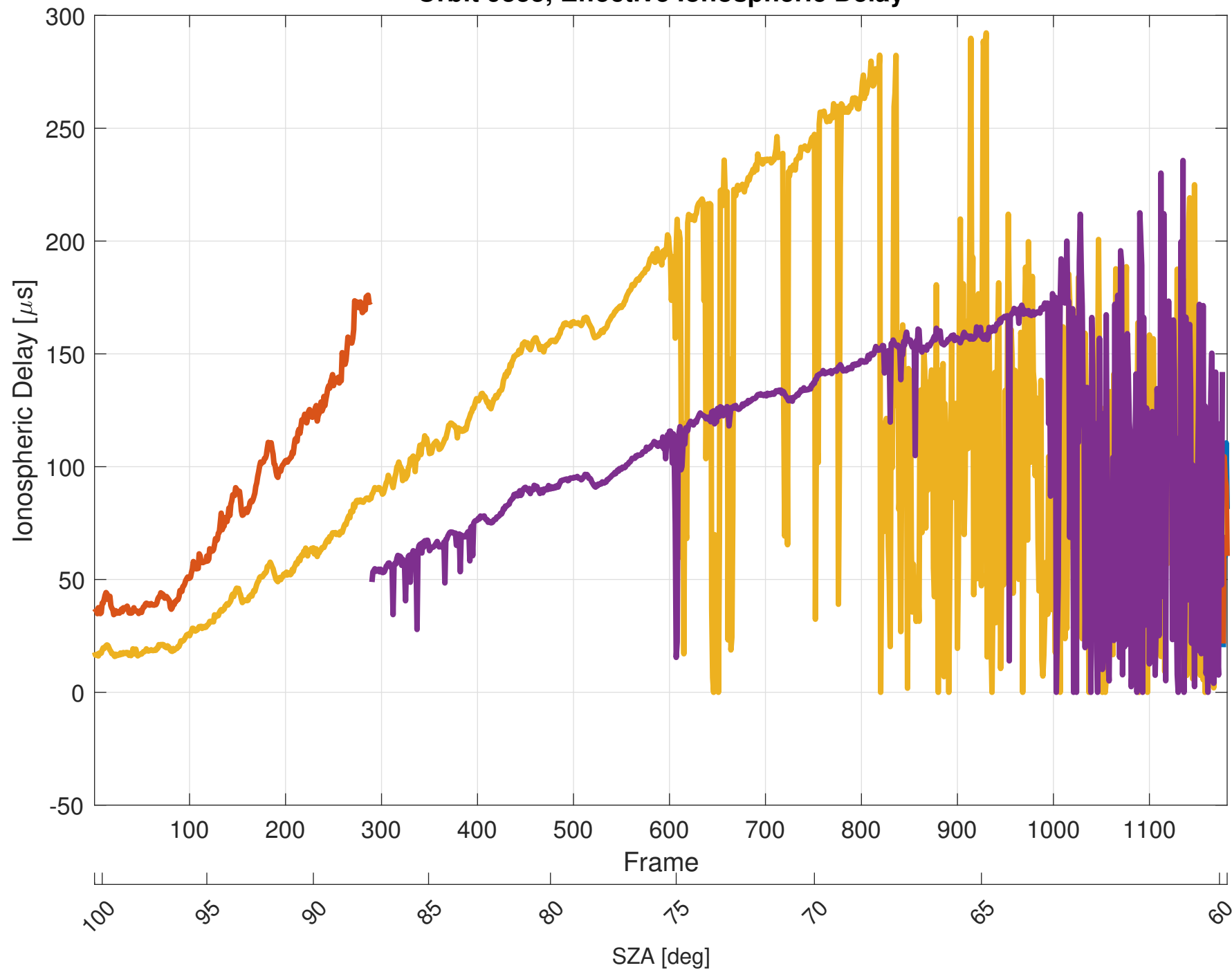
Orbit 9355, Effective Ionospheric Delay
