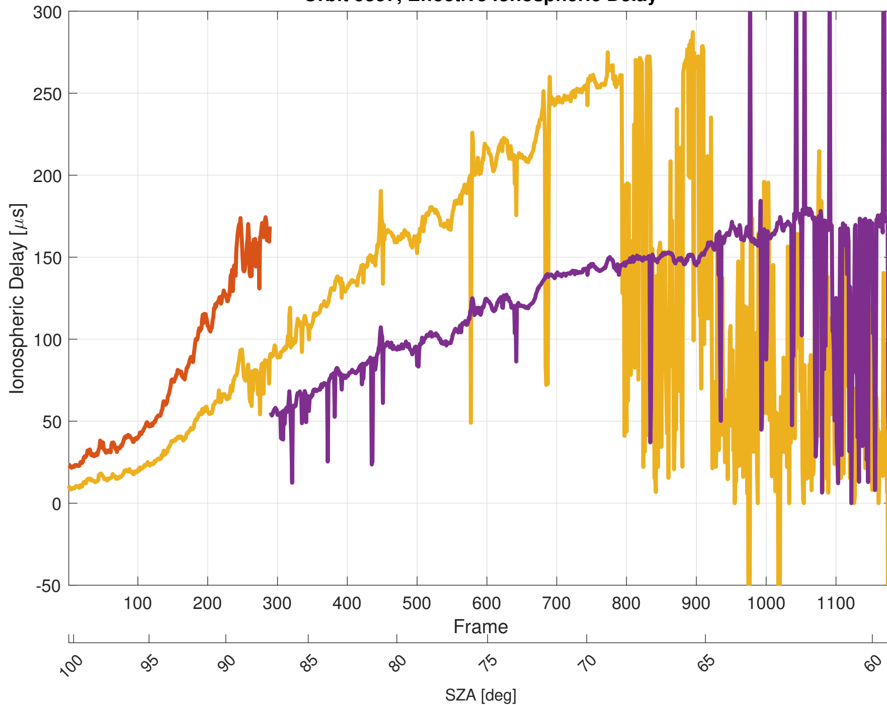
Orbit 9357, Effective Ionospheric Delay
