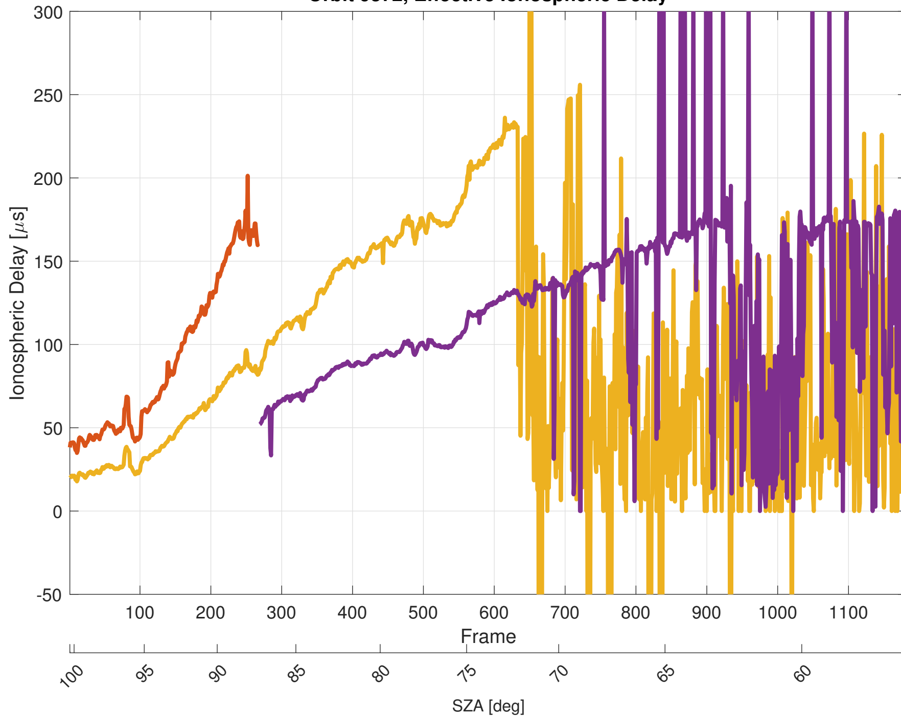
Orbit 9372, Effective Ionospheric Delay
