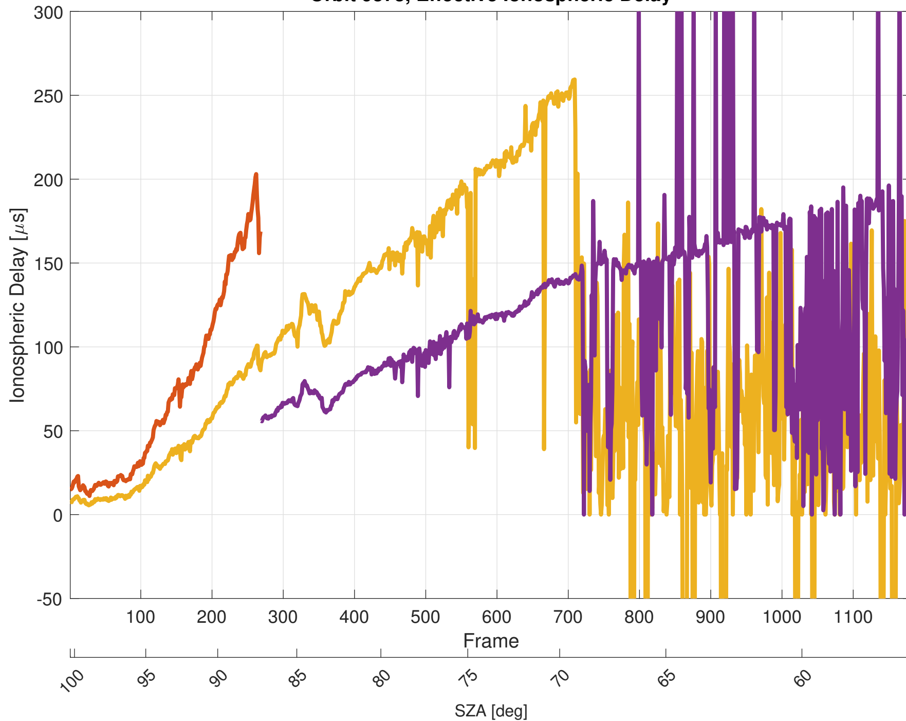
Orbit 9373, Effective Ionospheric Delay
