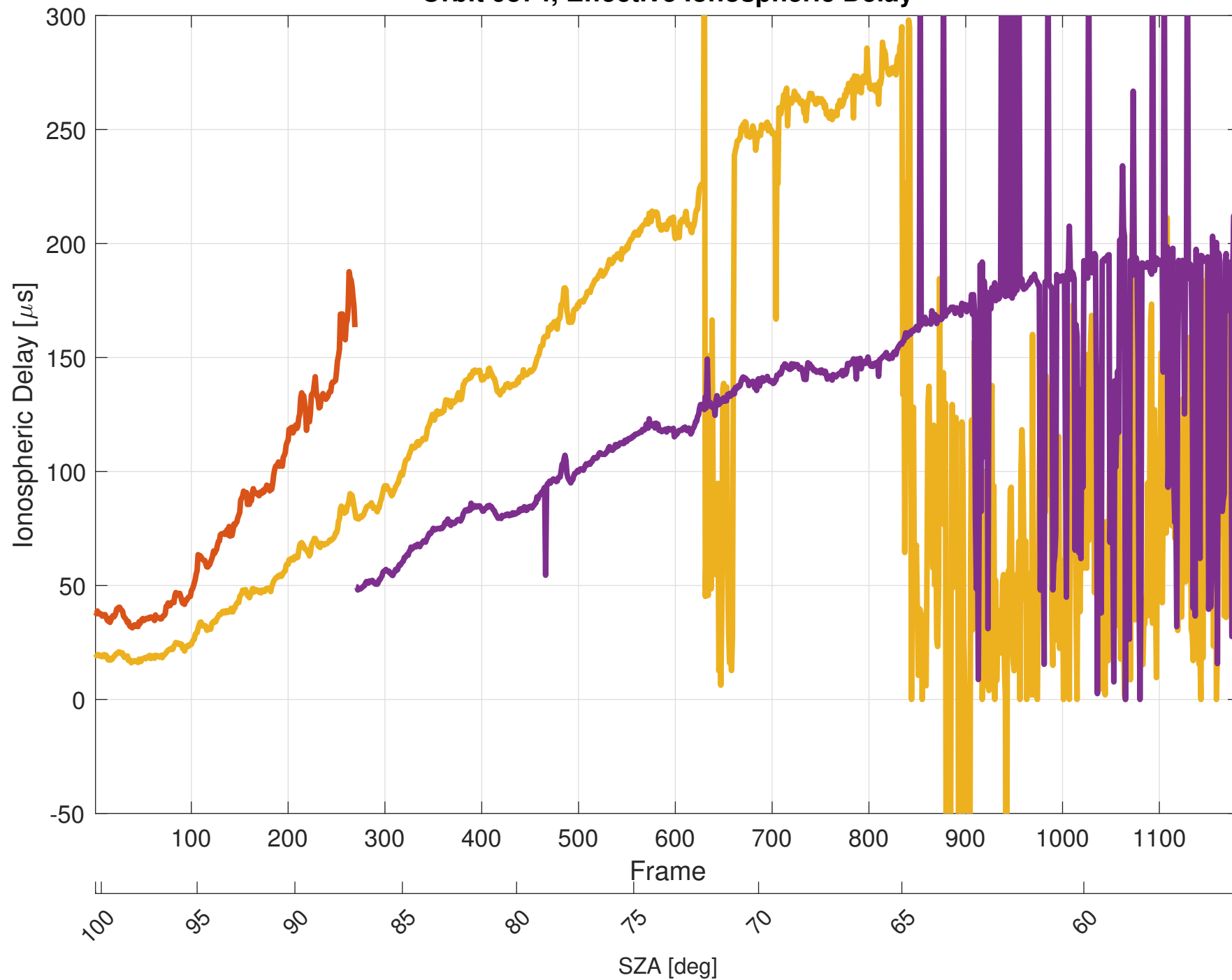
Orbit 9374, Effective Ionospheric Delay
