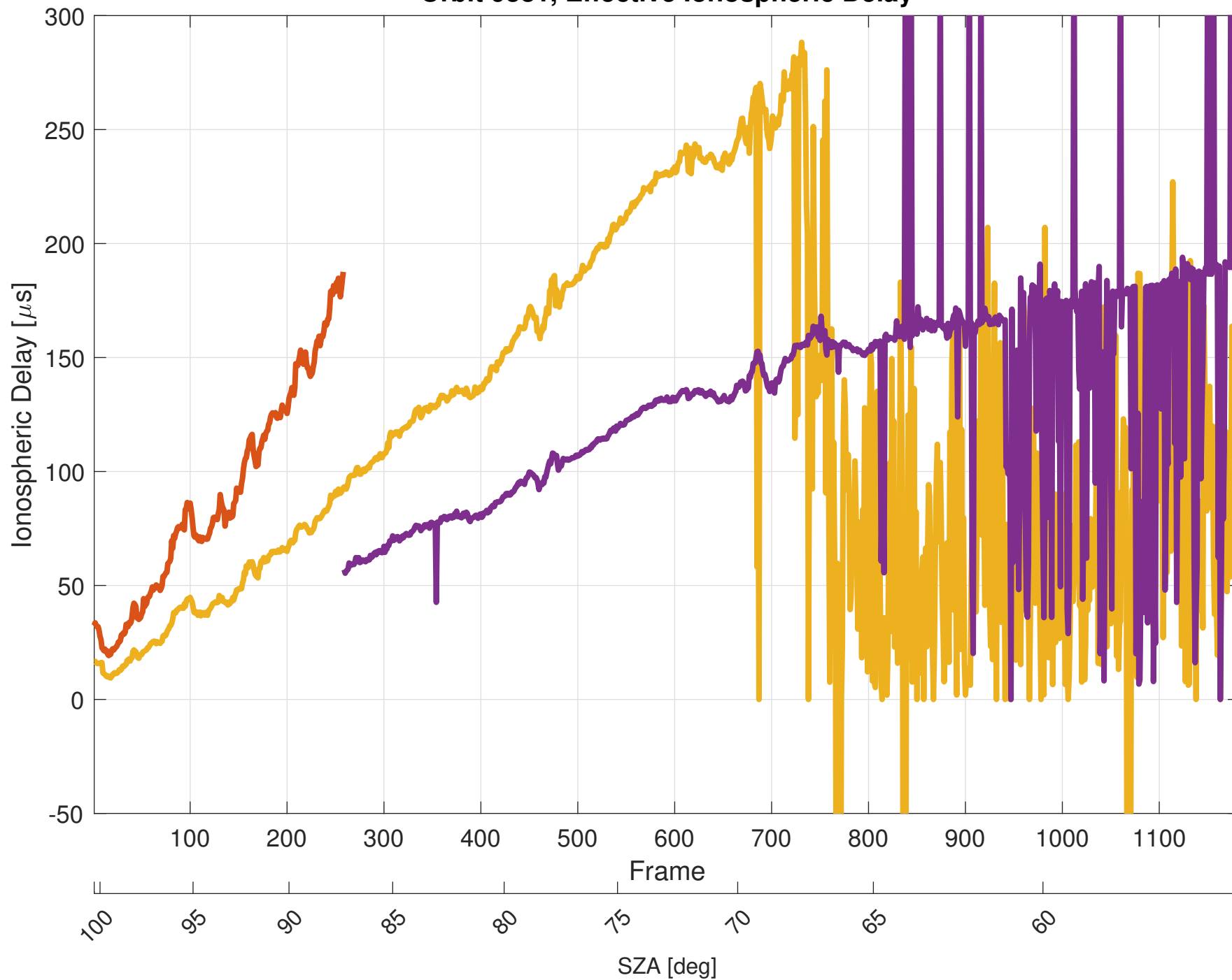
Orbit 9381, Effective Ionospheric Delay
