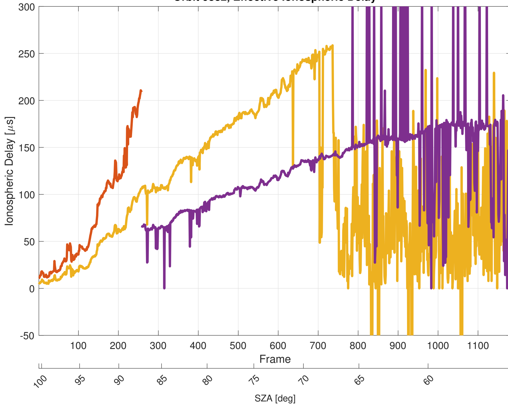
Orbit 9382, Effective Ionospheric Delay
