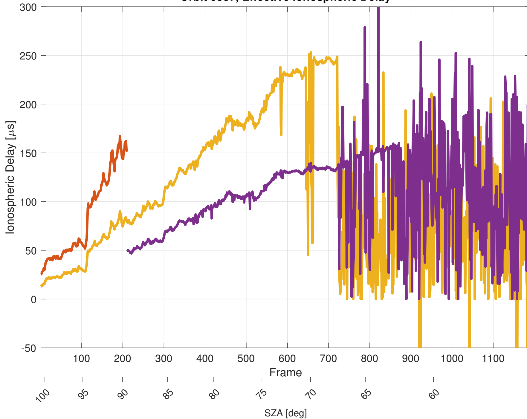
Orbit 9387, Effective Ionospheric Delay
