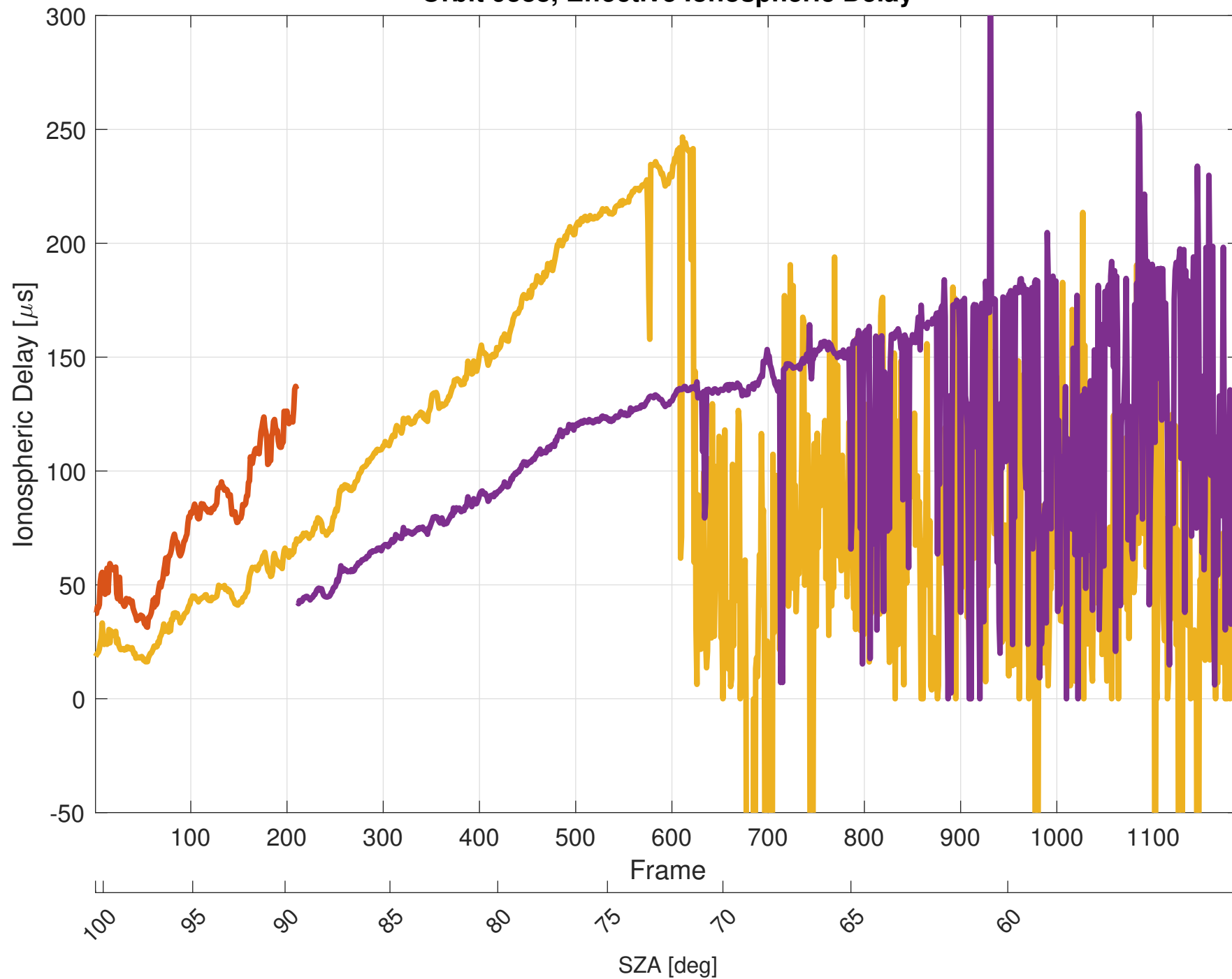
Orbit 9388, Effective Ionospheric Delay
