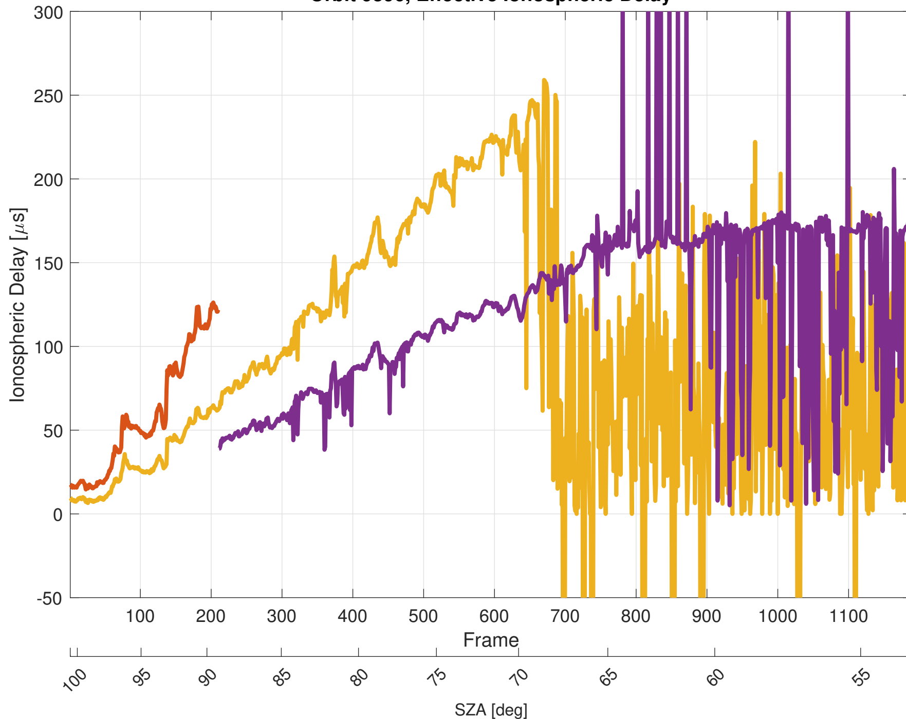
Orbit 9396, Effective Ionospheric Delay
