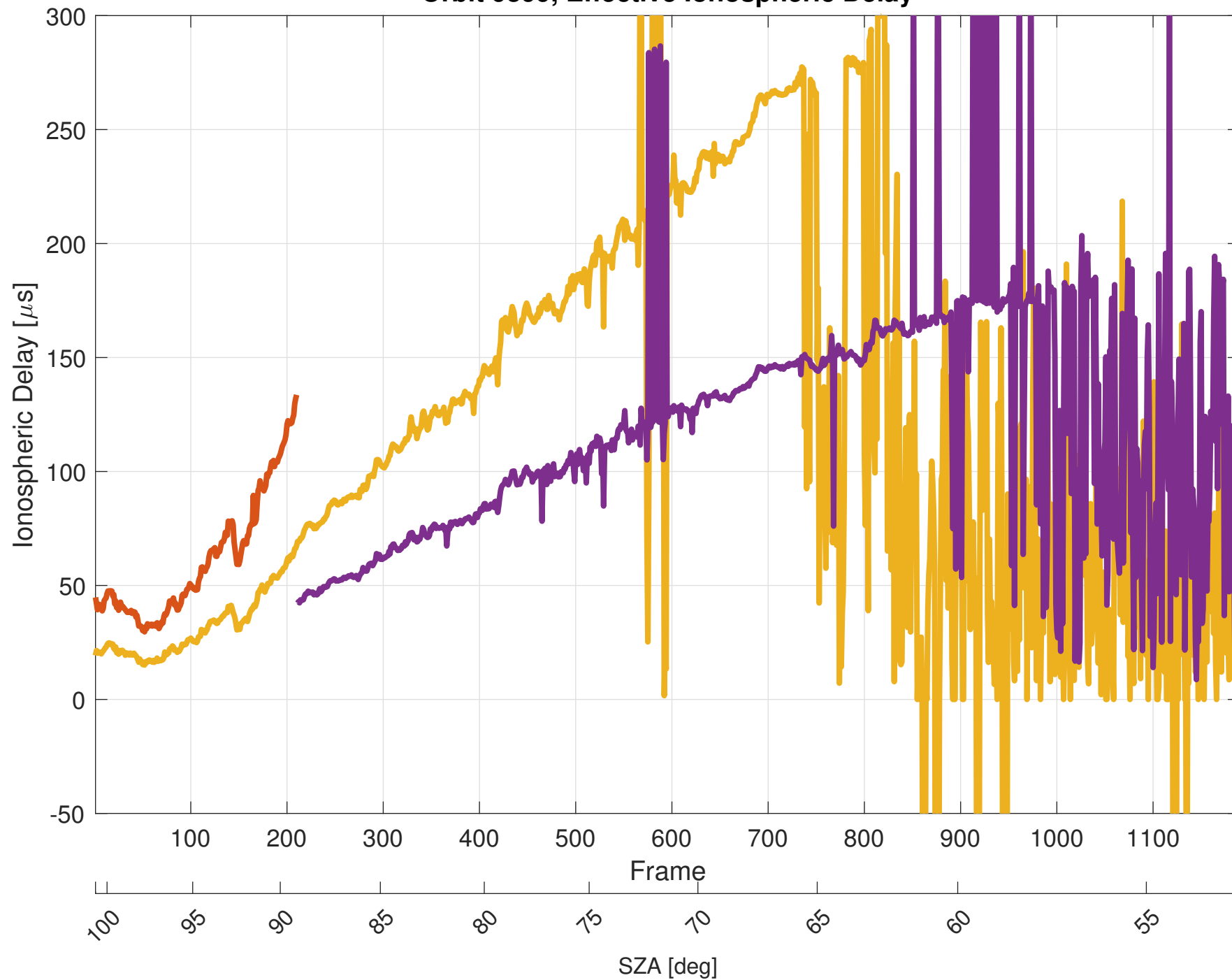
Orbit 9399, Effective Ionospheric Delay
