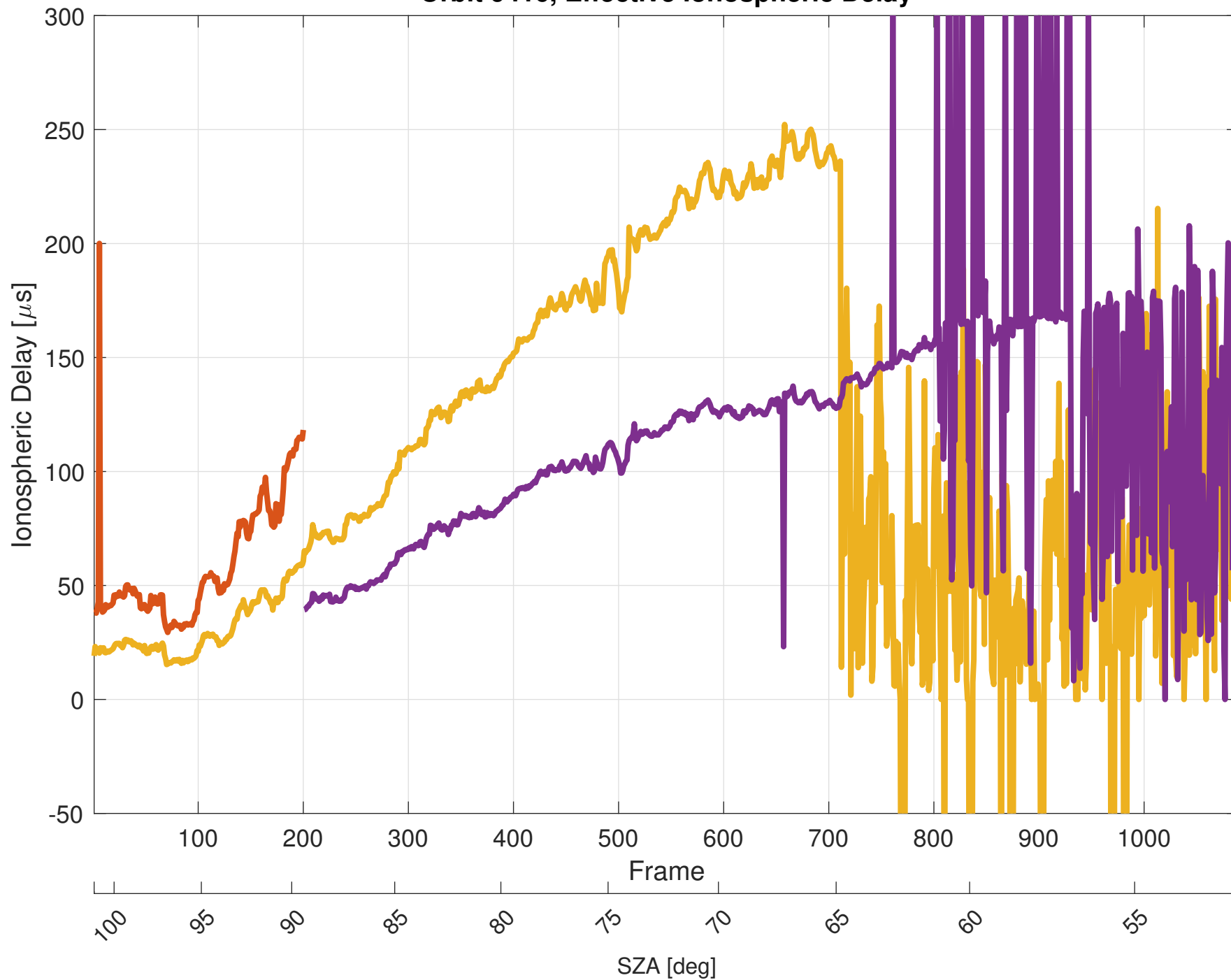
Orbit 9416, Effective Ionospheric Delay
