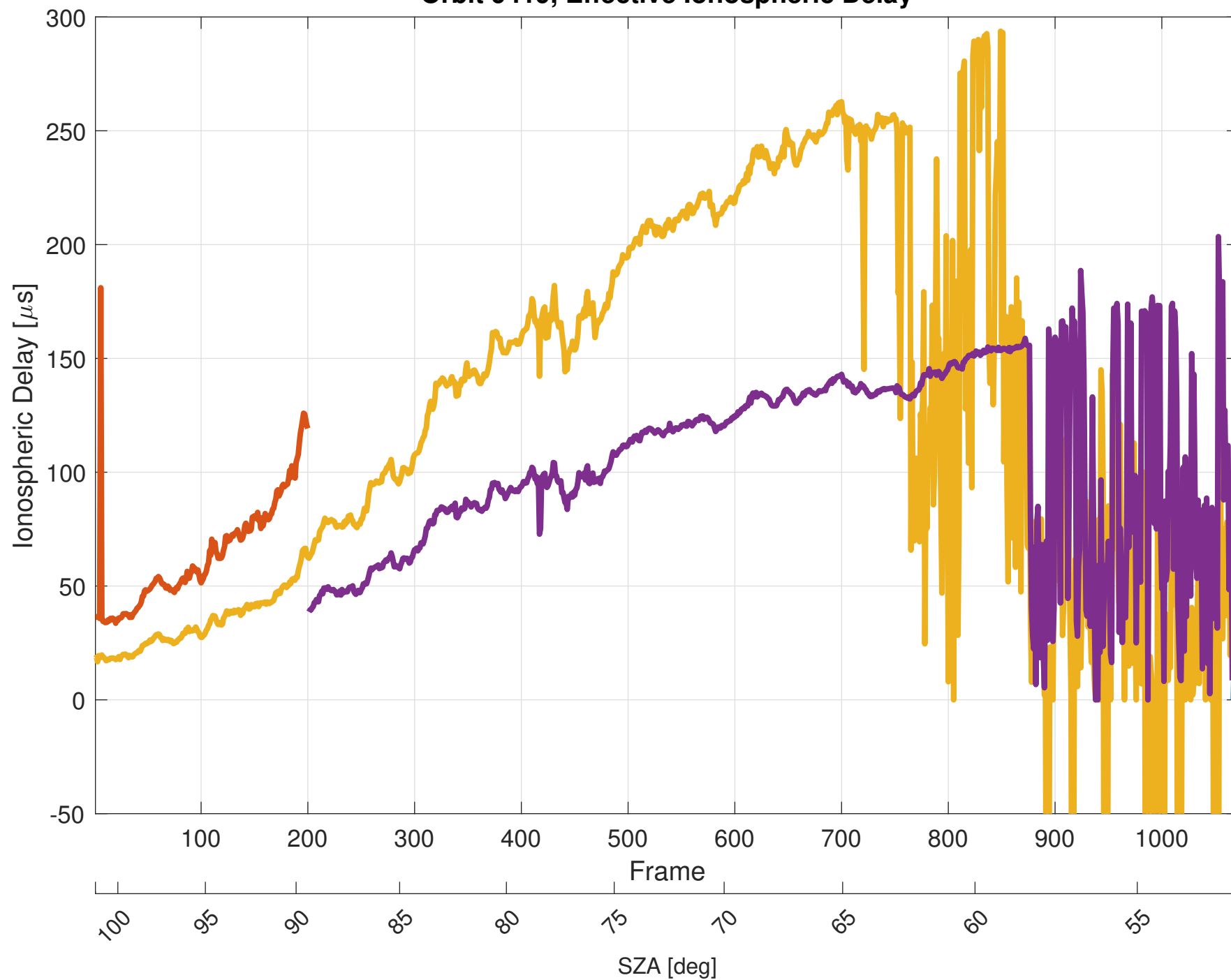
Orbit 9419, Effective Ionospheric Delay
