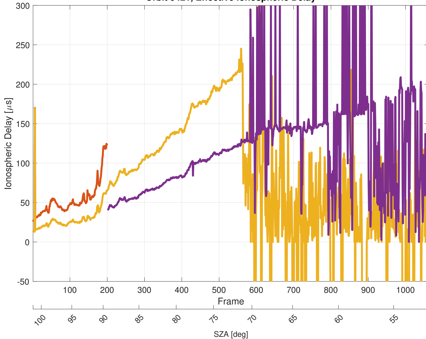
Orbit 9421, Effective Ionospheric Delay
