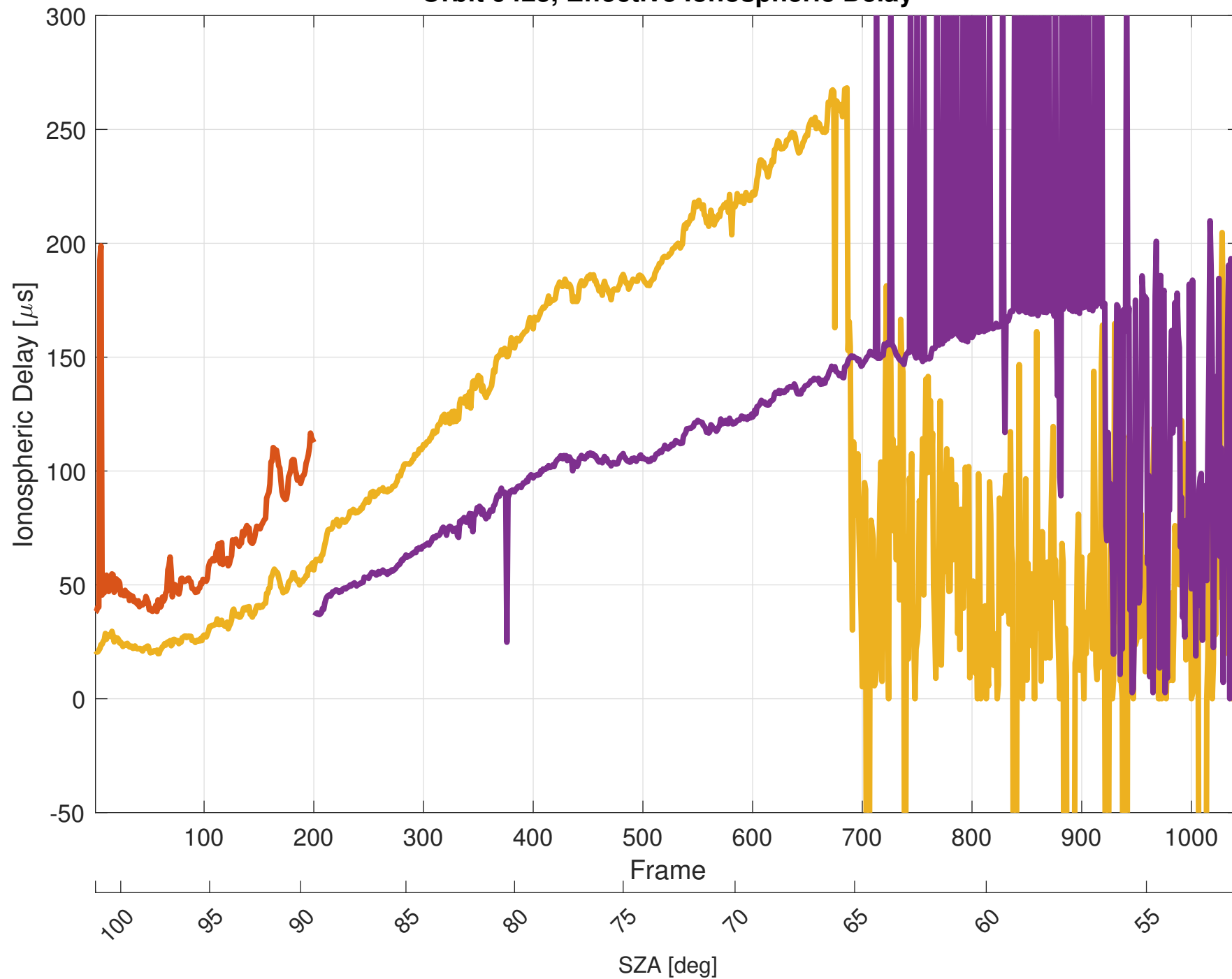
Orbit 9423, Effective Ionospheric Delay
