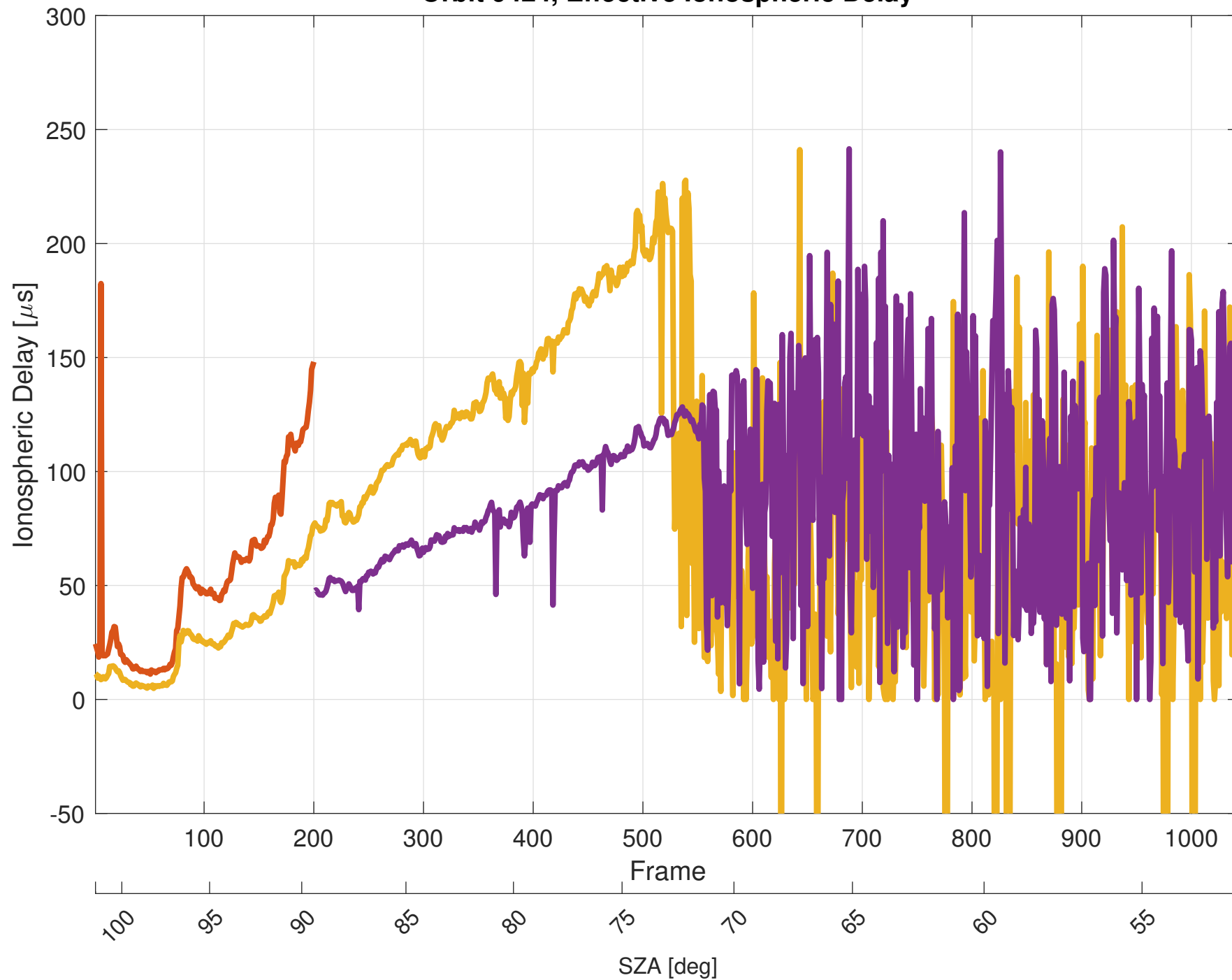
Orbit 9424, Effective Ionospheric Delay
