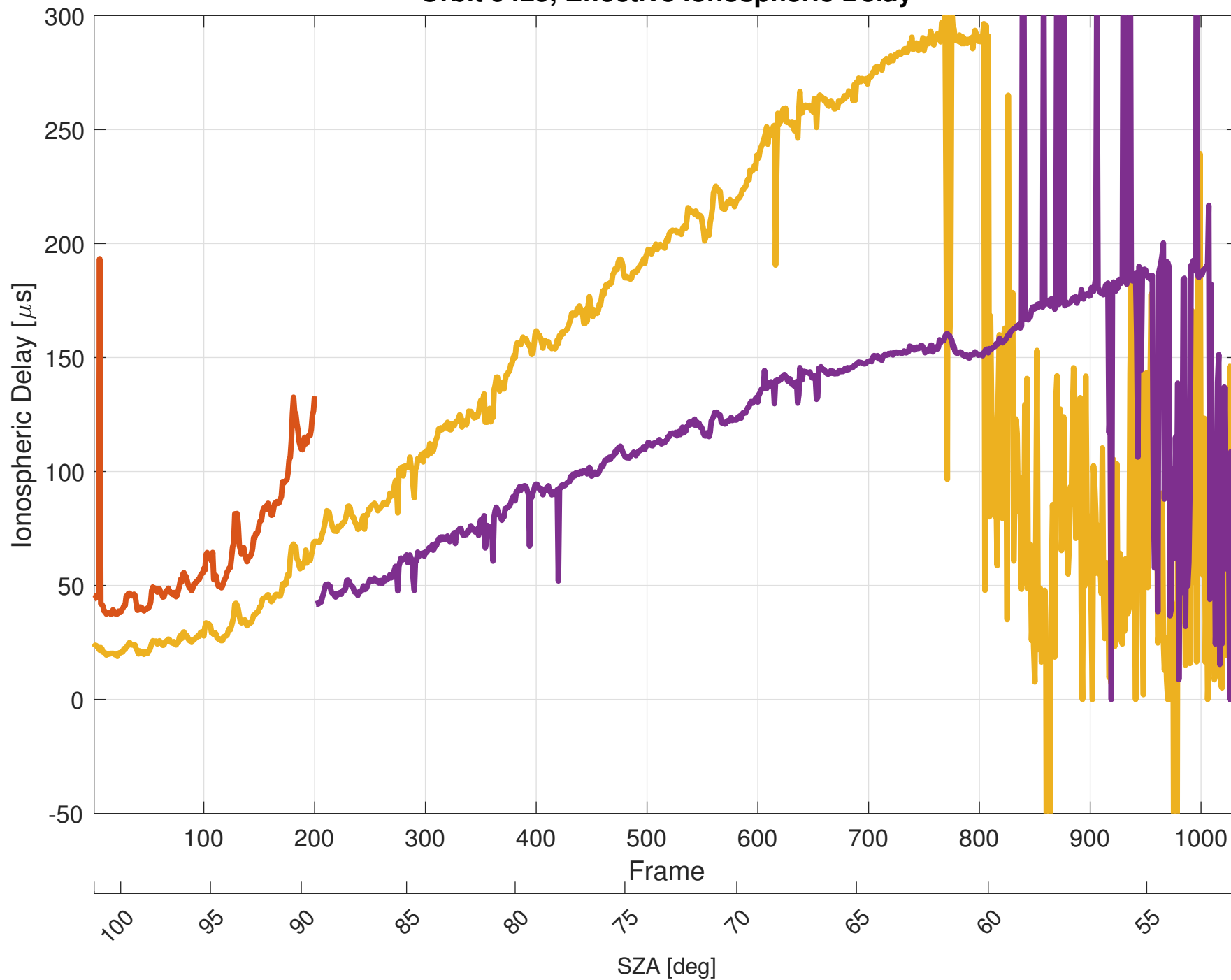
Orbit 9425, Effective Ionospheric Delay
