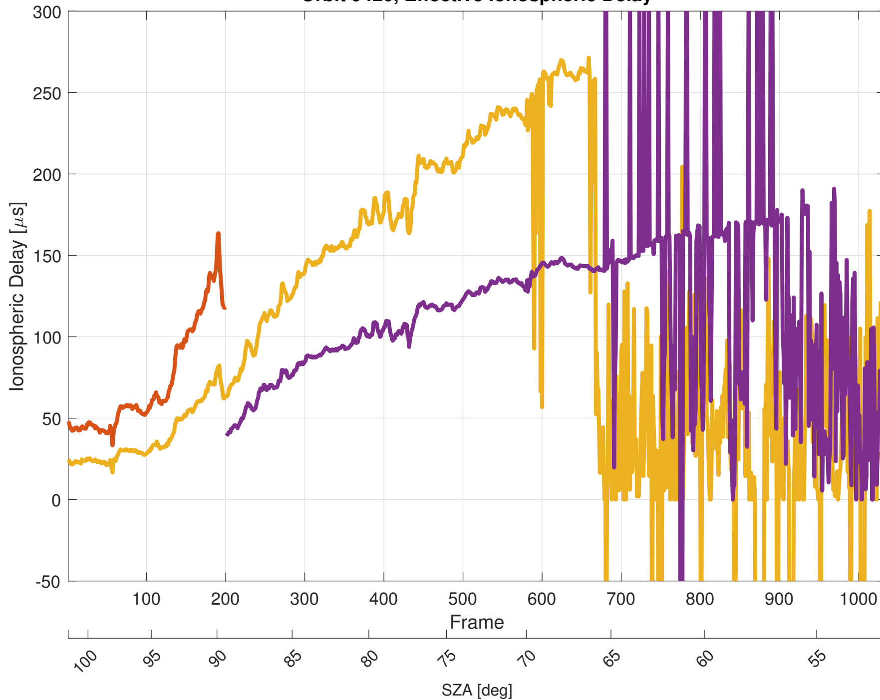
Orbit 9426, Effective Ionospheric Delay
