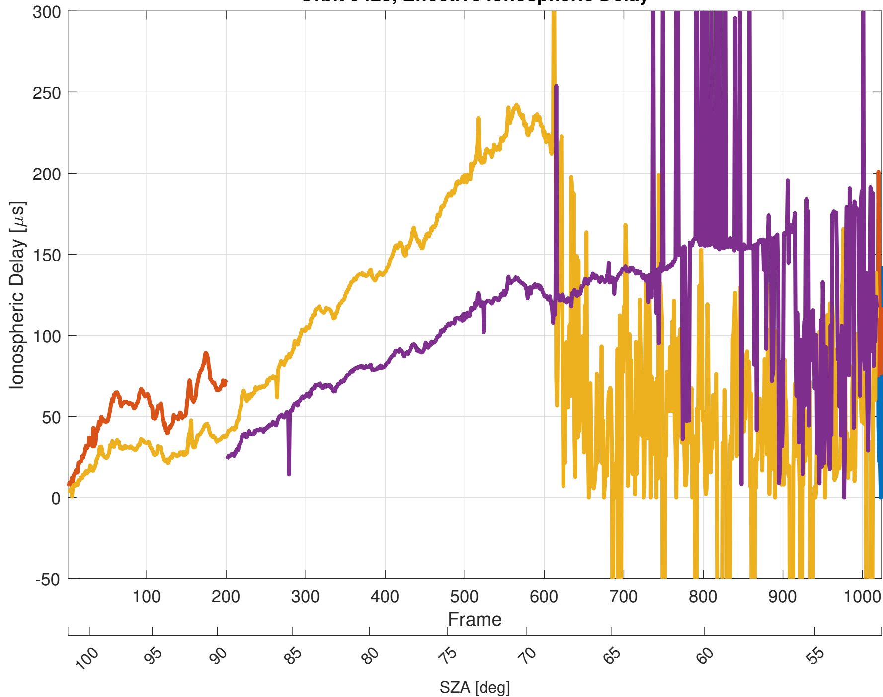
Orbit 9428, Effective Ionospheric Delay
