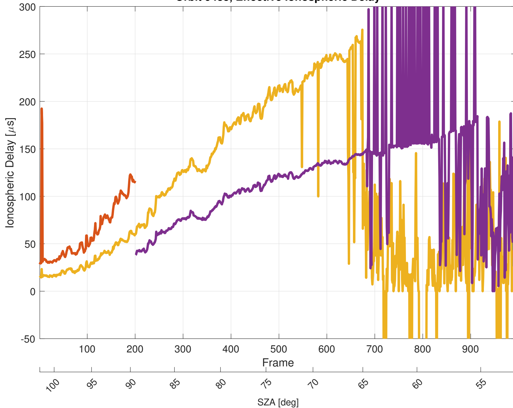
Orbit 9433, Effective Ionospheric Delay
