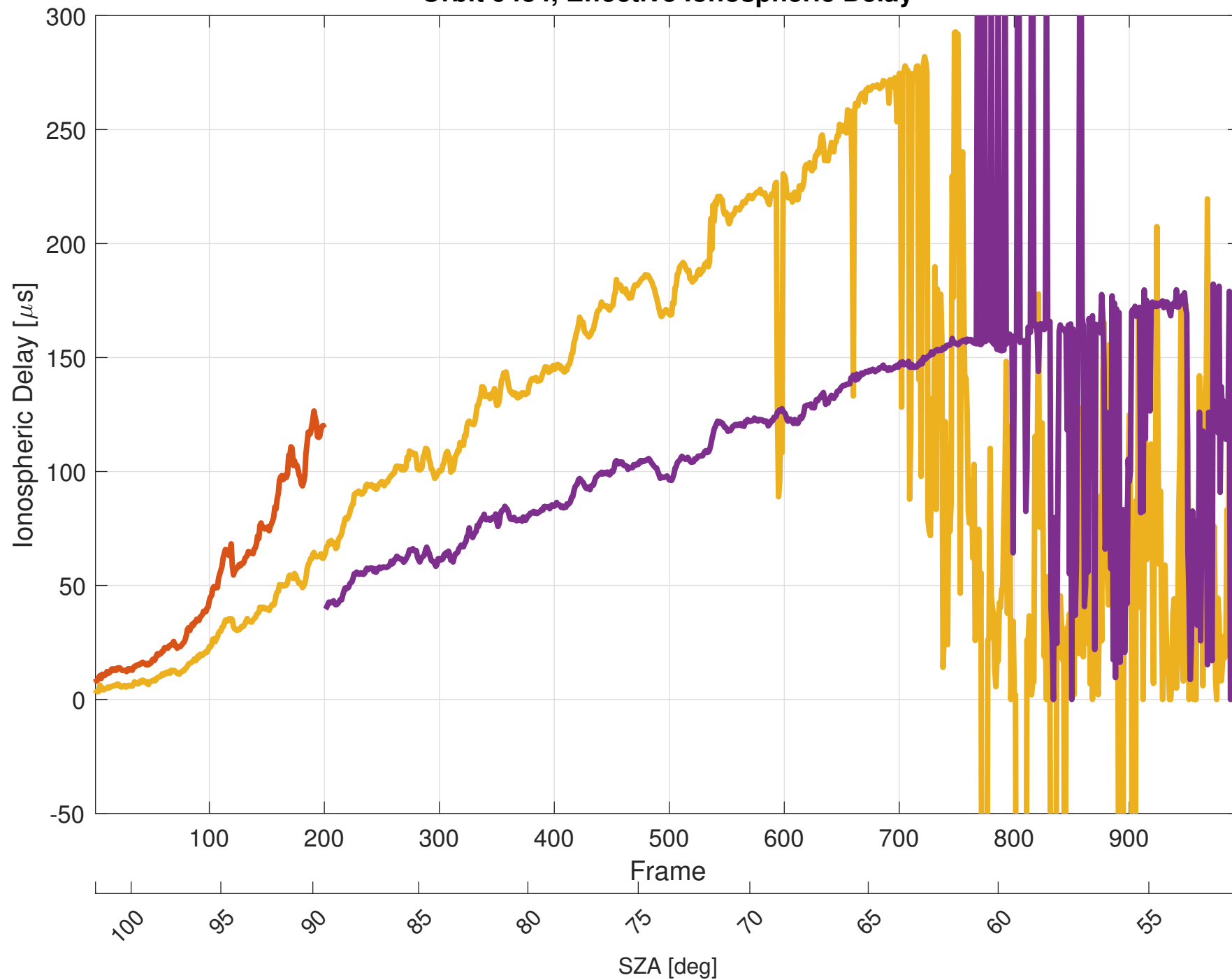
Orbit 9434, Effective Ionospheric Delay
