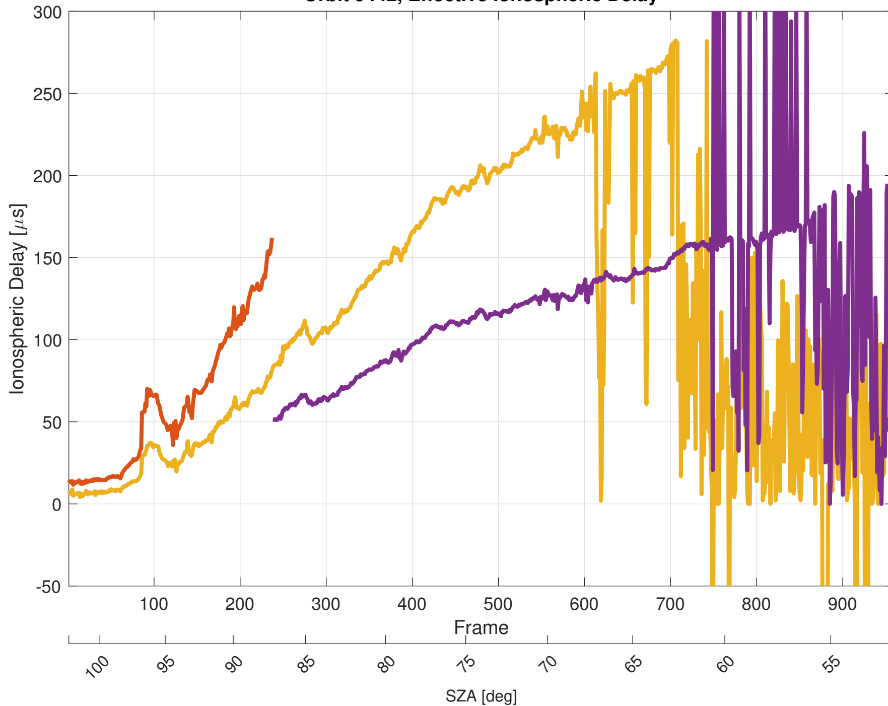
Orbit 9442, Effective Ionospheric Delay
