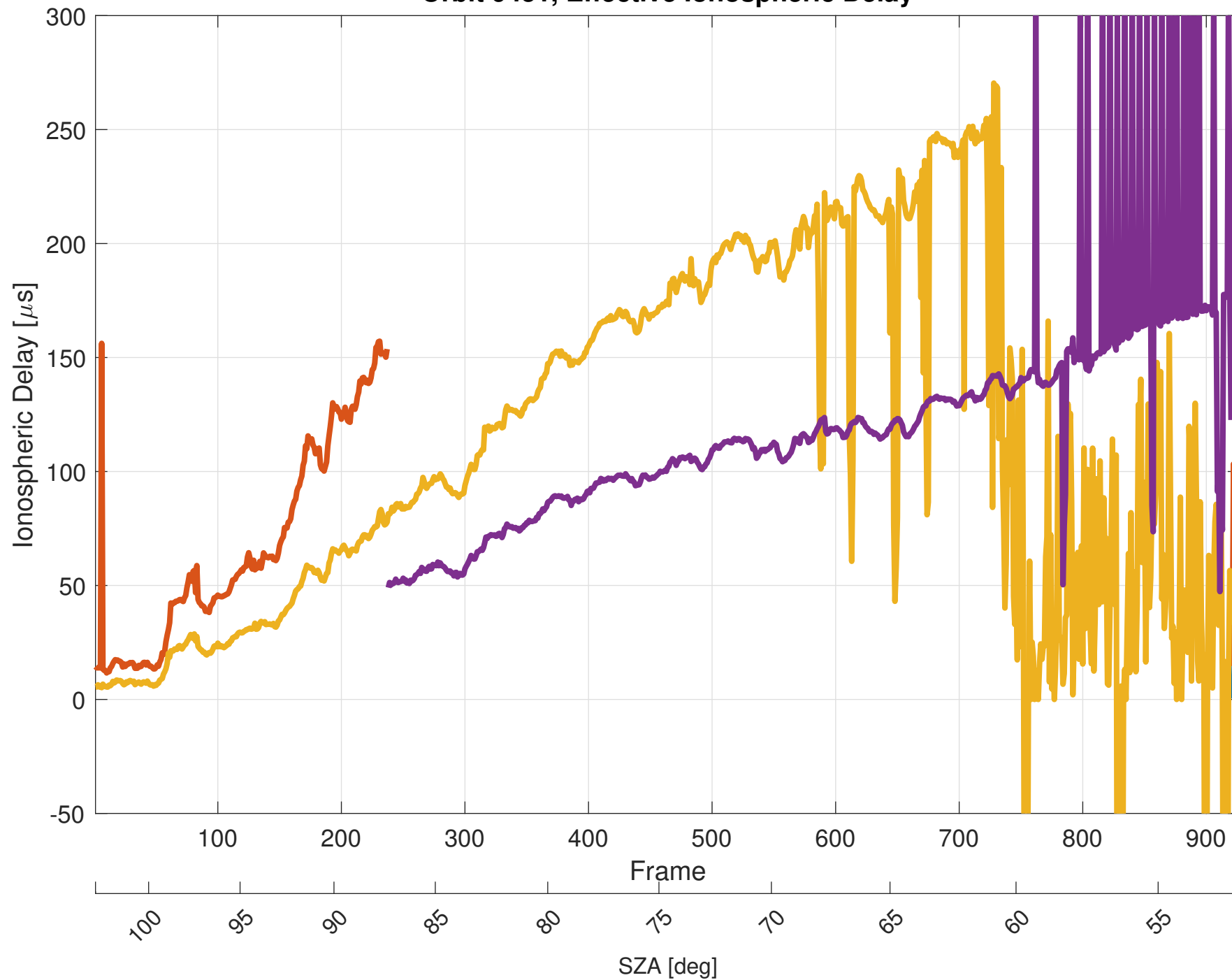
Orbit 9451, Effective Ionospheric Delay
