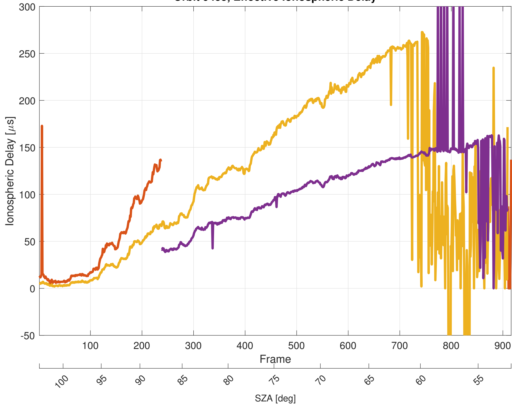
Orbit 9455, Effective Ionospheric Delay
