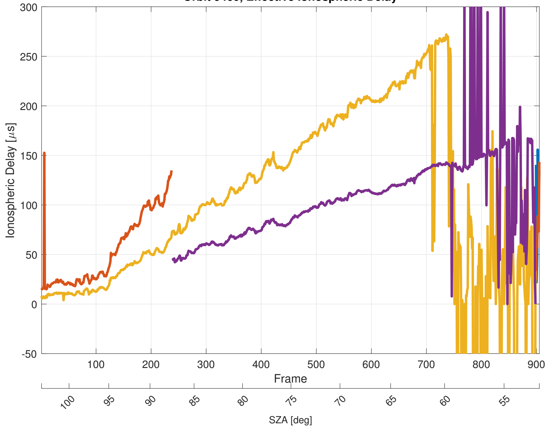
Orbit 9460, Effective Ionospheric Delay
