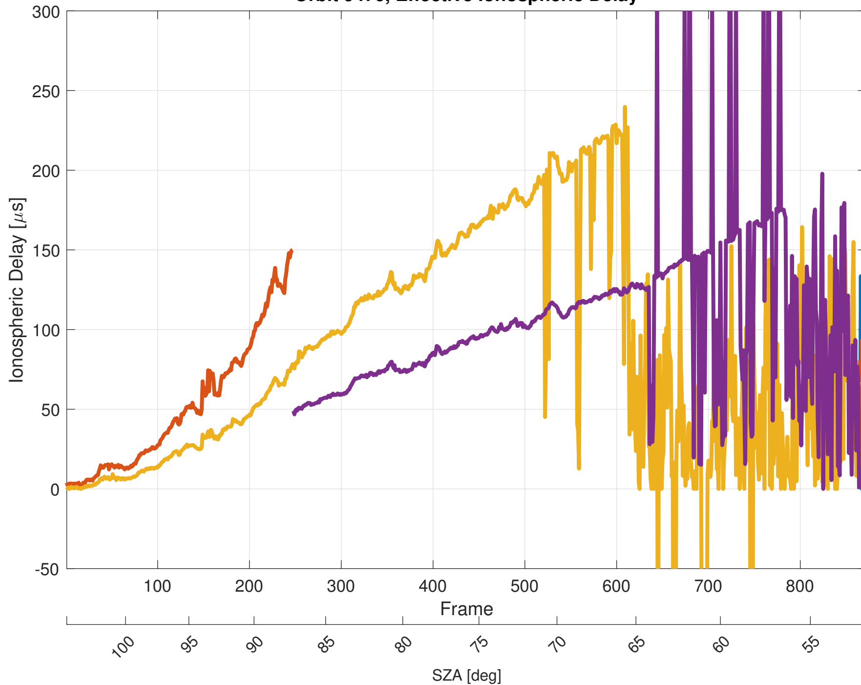
Orbit 9476, Effective Ionospheric Delay
