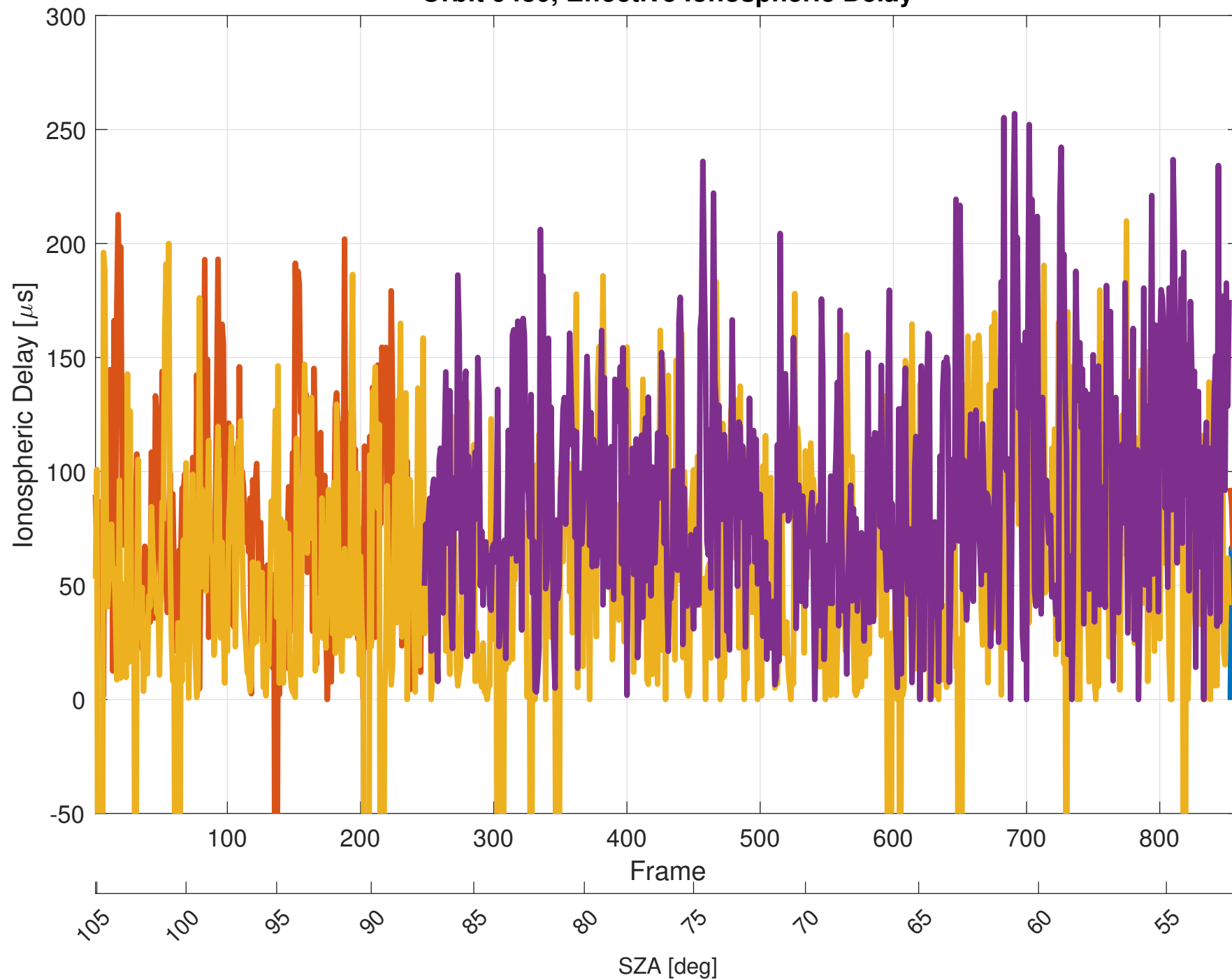
Orbit 9480, Effective Ionospheric Delay
