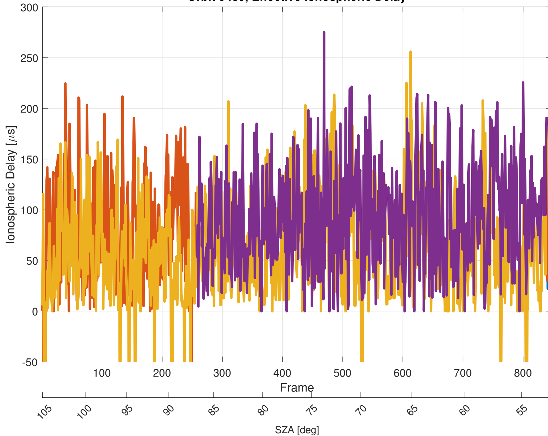
Orbit 9485, Effective Ionospheric Delay
