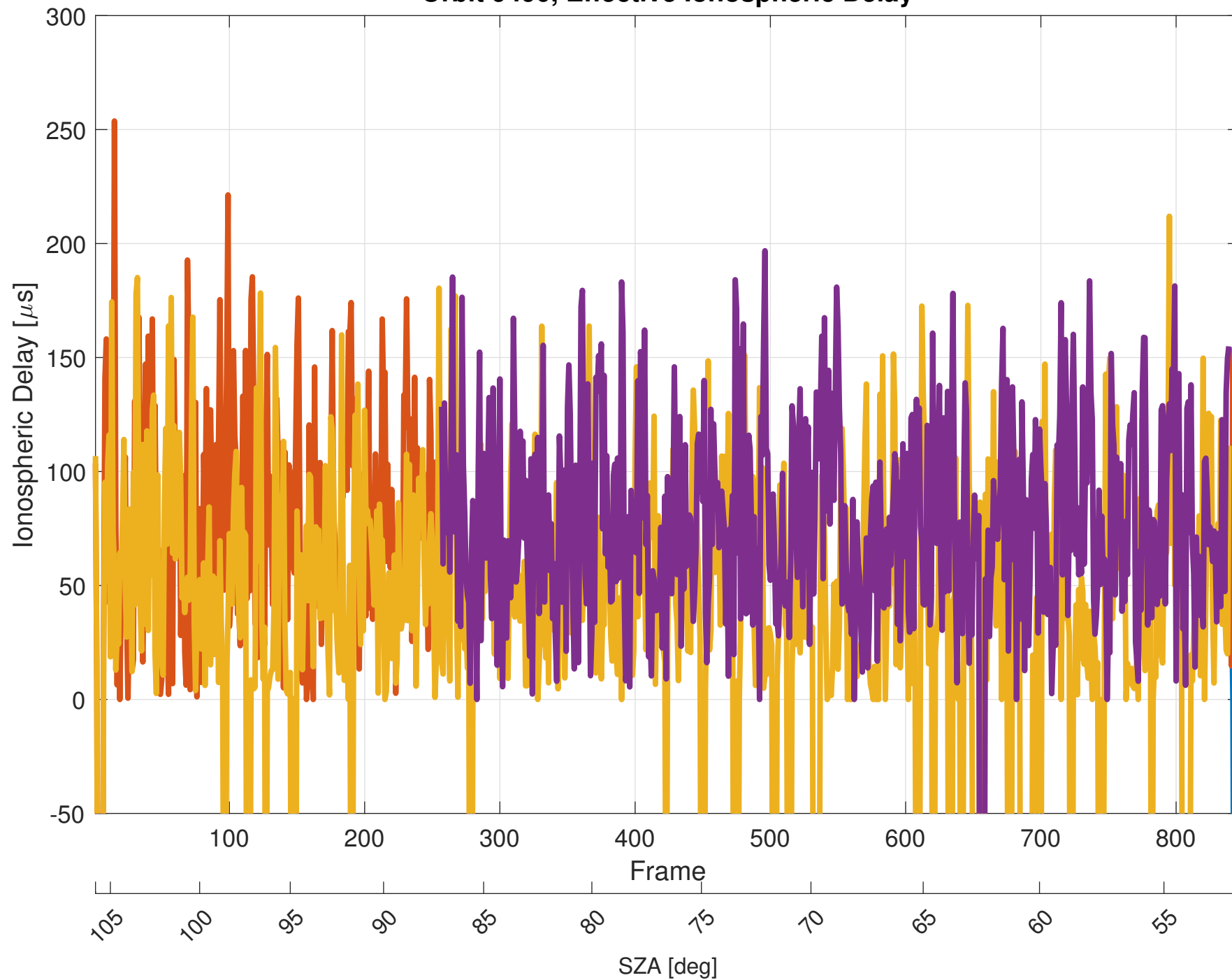
Orbit 9490, Effective Ionospheric Delay
