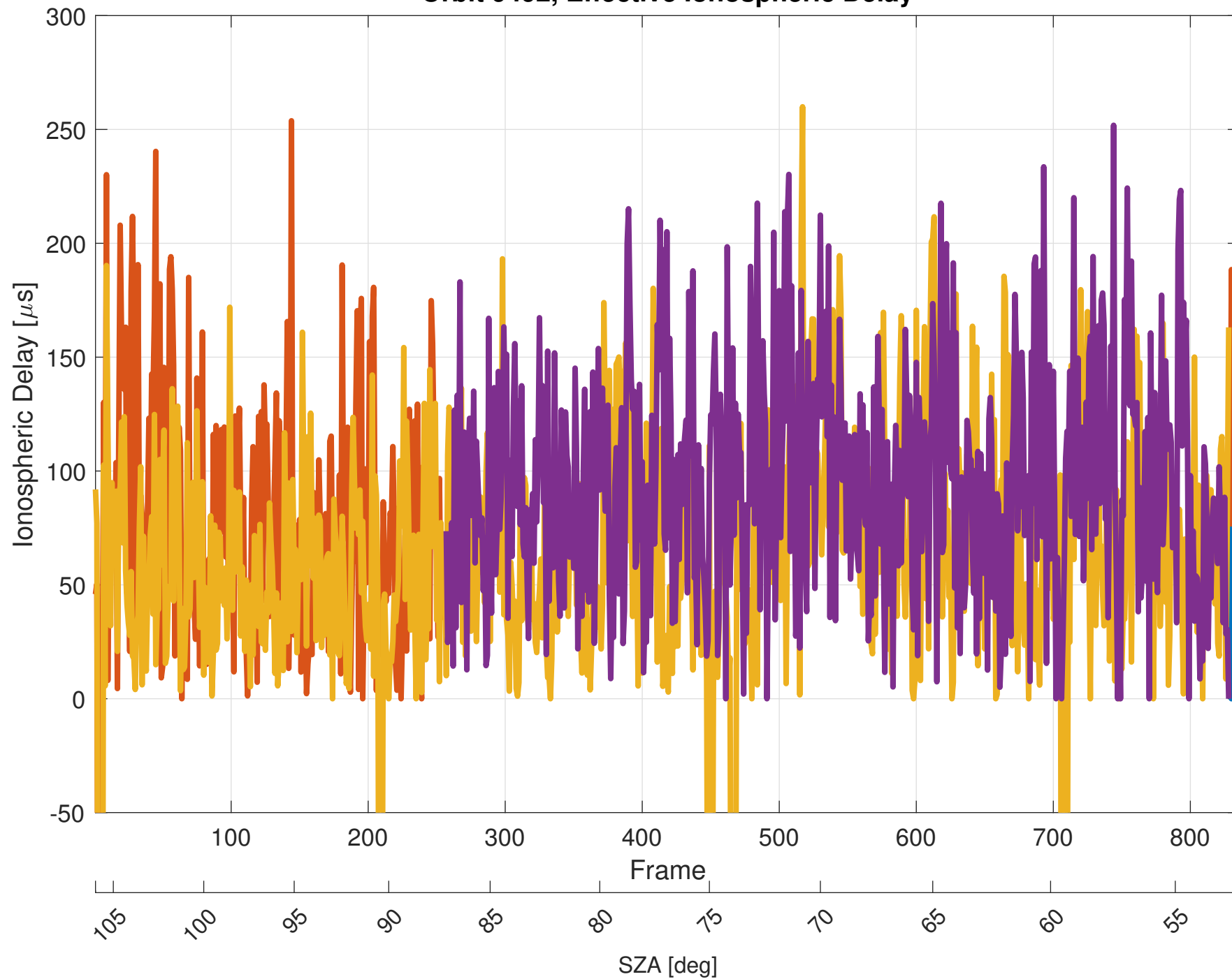
Orbit 9492, Effective Ionospheric Delay
