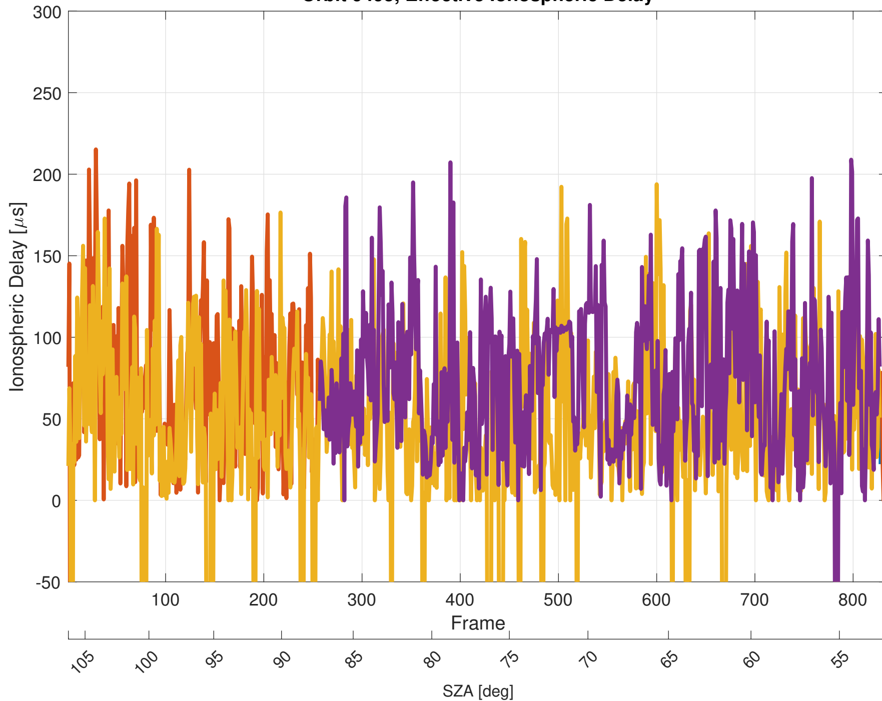
Orbit 9495, Effective Ionospheric Delay
