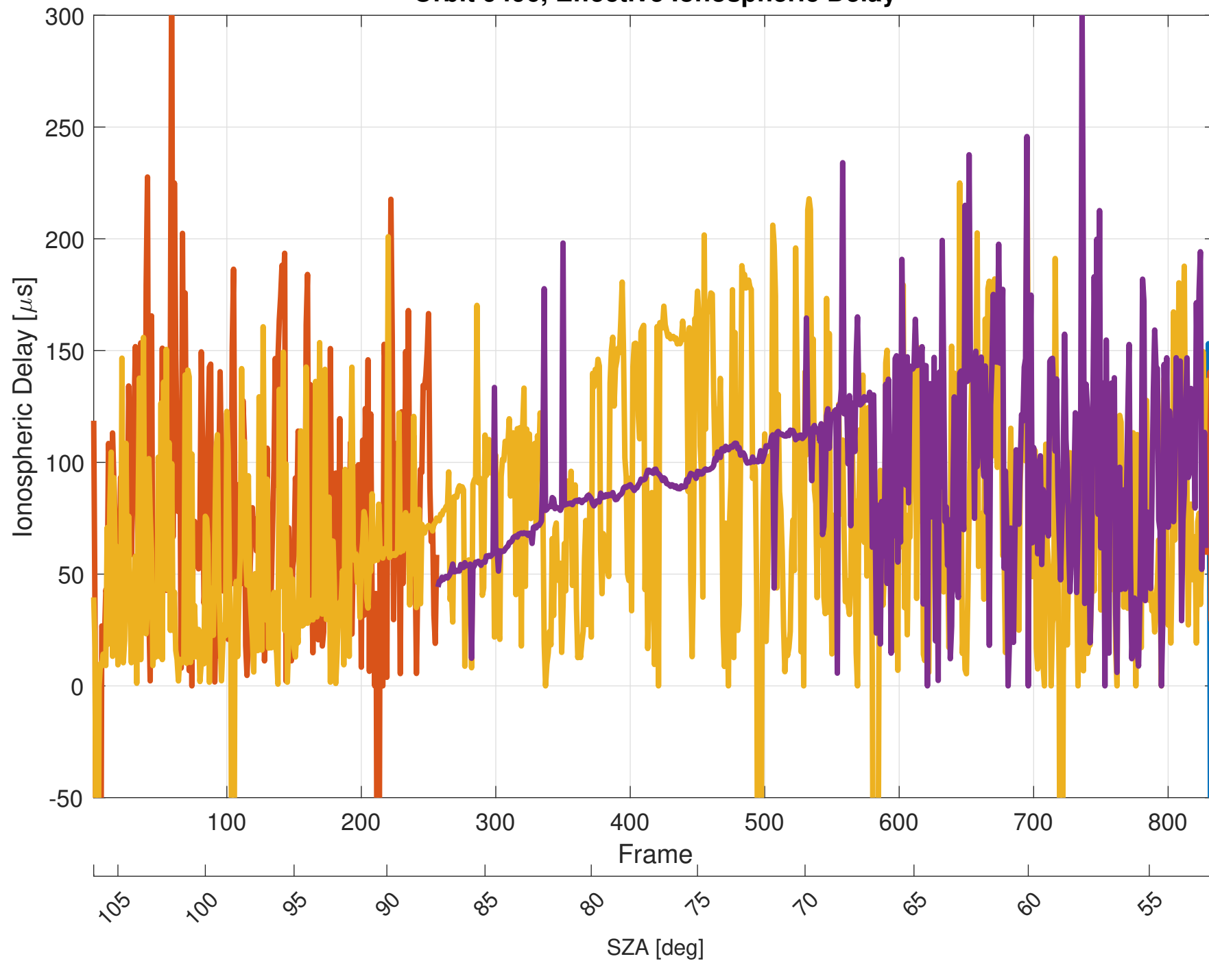
Orbit 9496, Effective Ionospheric Delay
