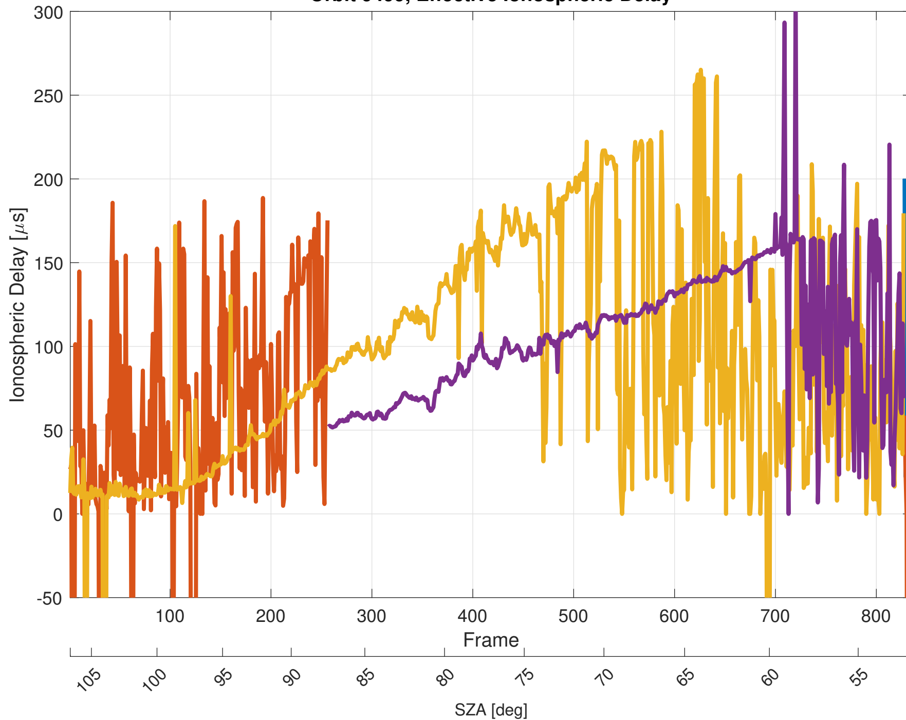
Orbit 9499, Effective Ionospheric Delay
