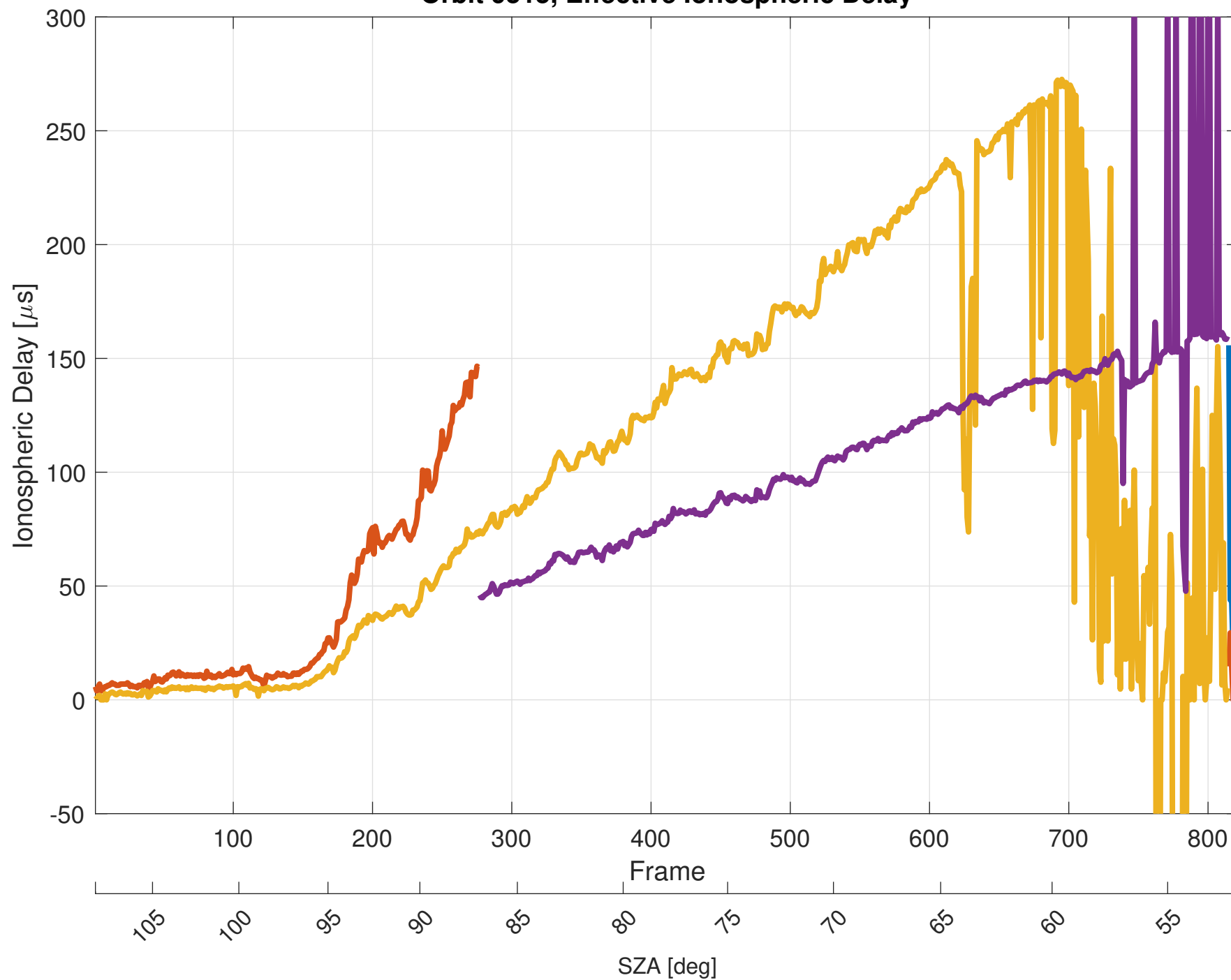
Orbit 9515, Effective Ionospheric Delay
