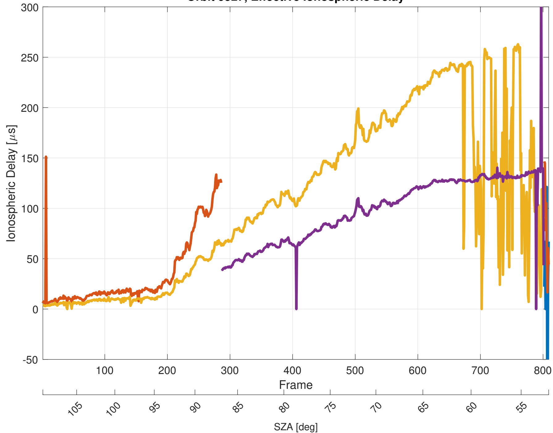
Orbit 9527, Effective Ionospheric Delay
