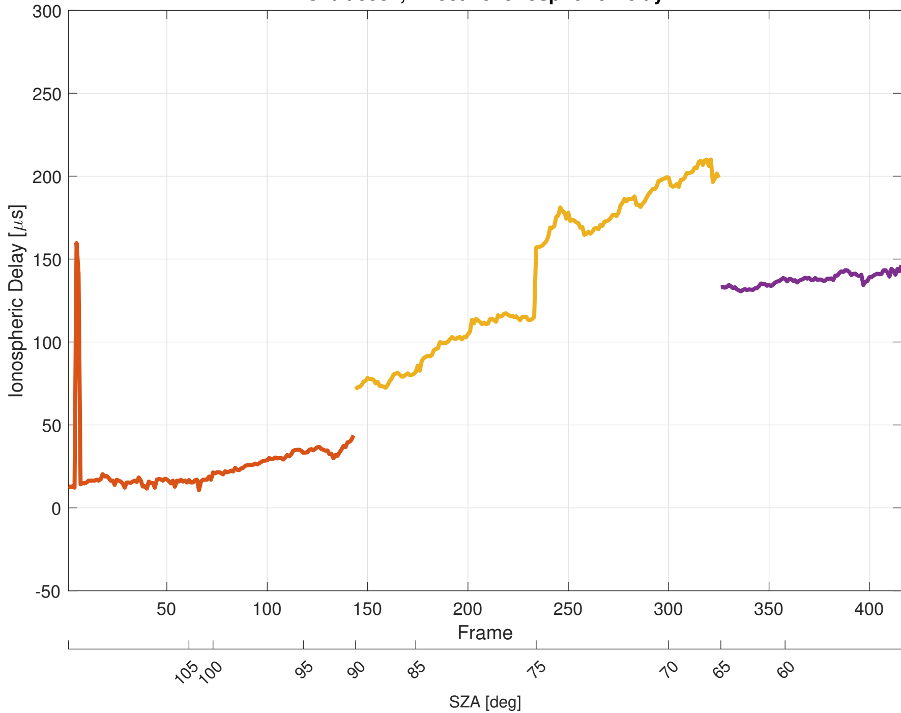
Orbit 9531, Effective Ionospheric Delay
