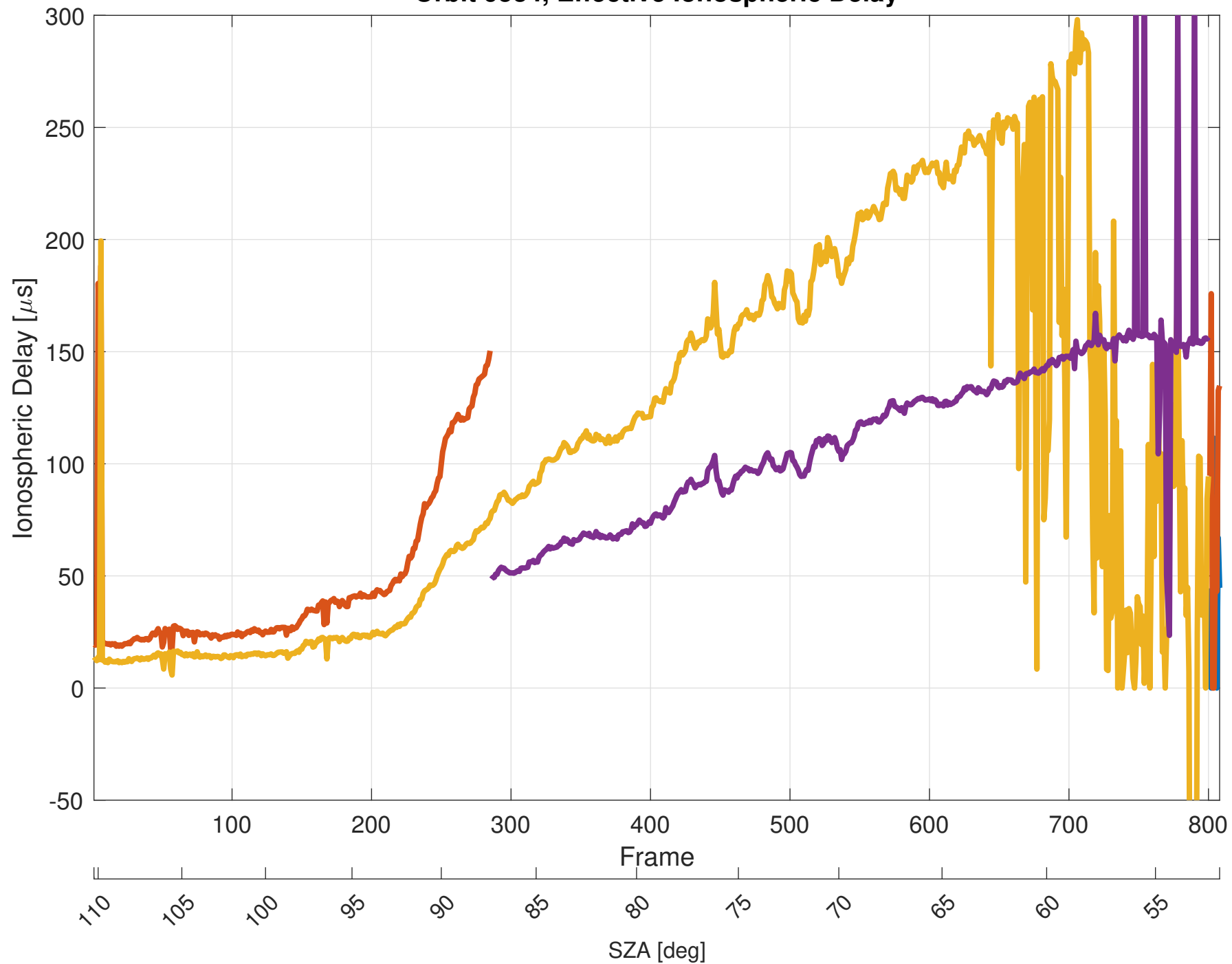
Orbit 9534, Effective Ionospheric Delay
