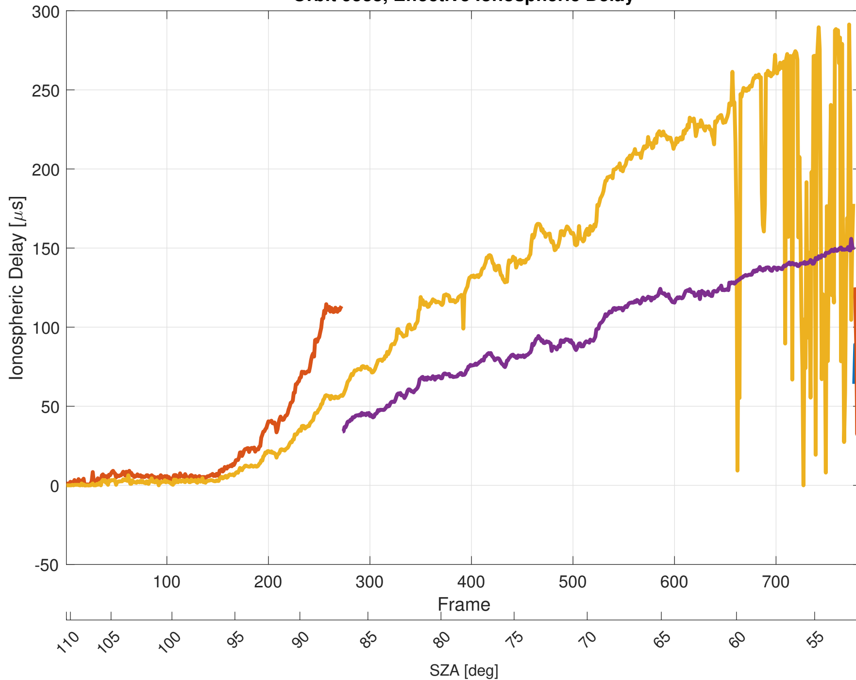
Orbit 9538, Effective Ionospheric Delay
