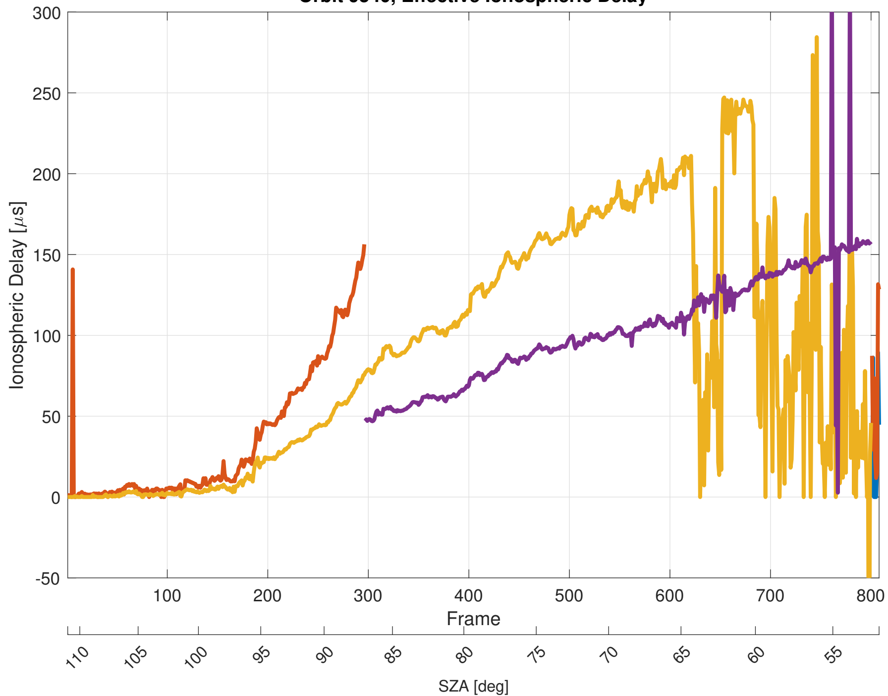
Orbit 9540, Effective Ionospheric Delay
