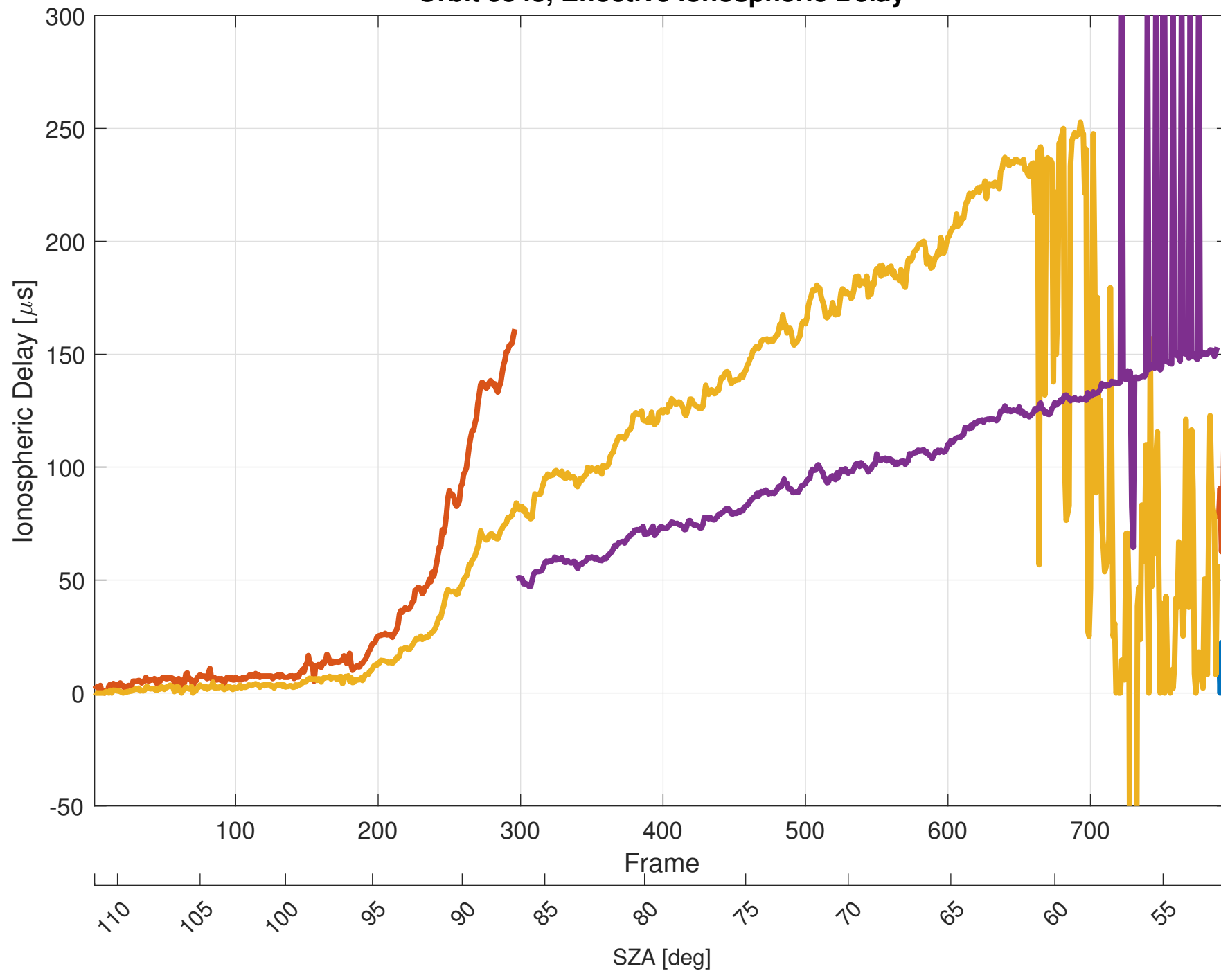
Orbit 9543, Effective Ionospheric Delay
