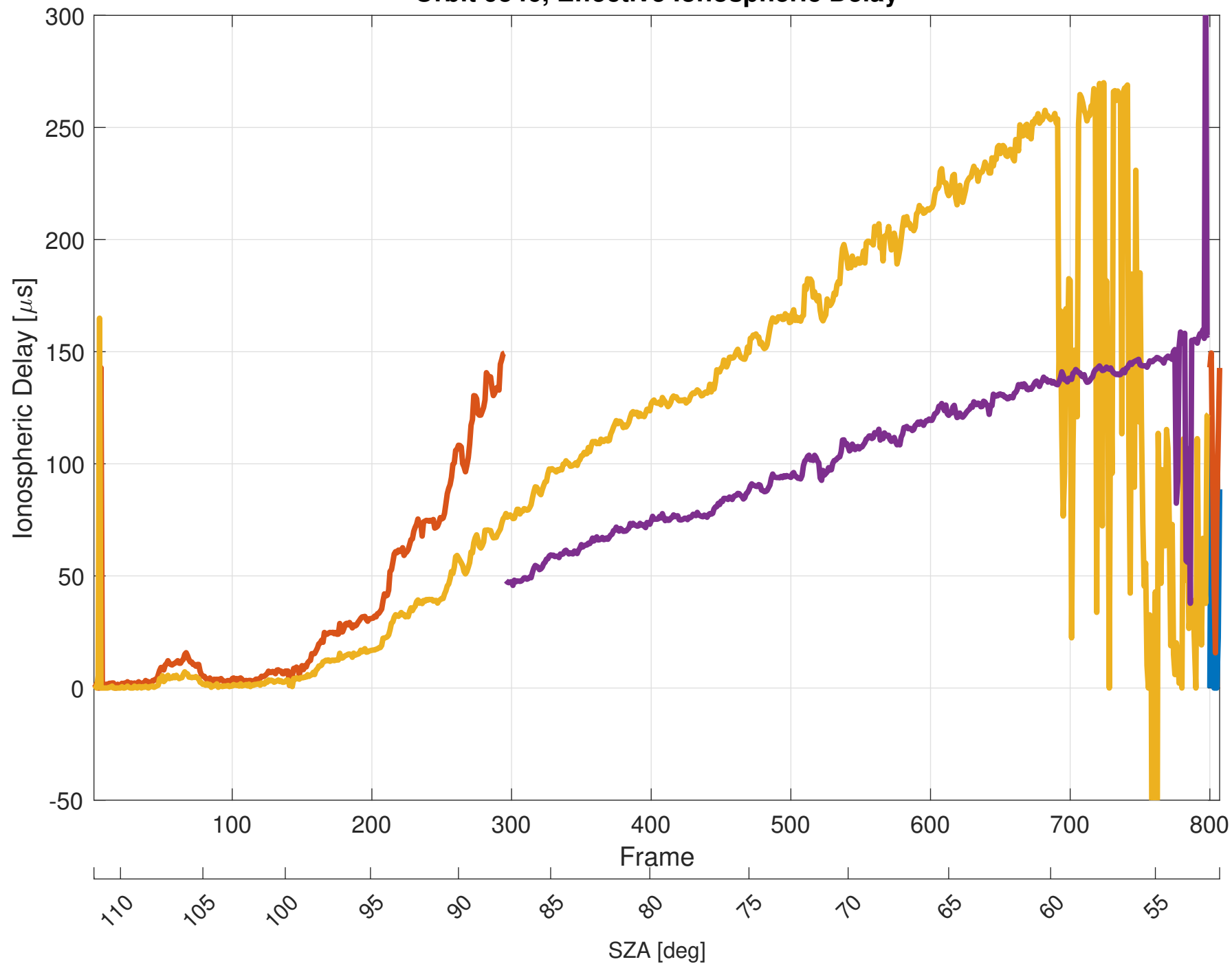
Orbit 9546, Effective Ionospheric Delay
