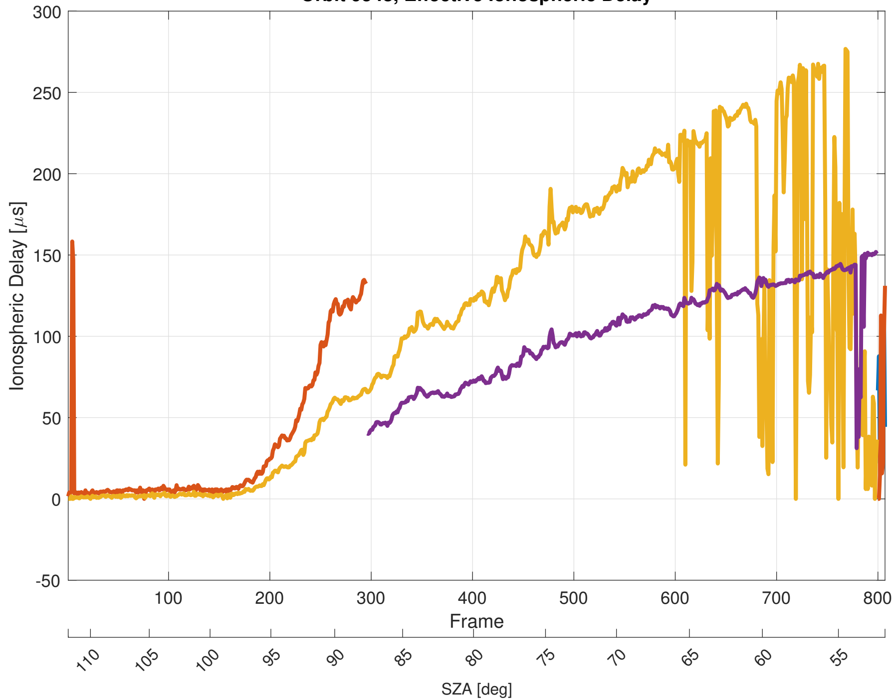
Orbit 9548, Effective Ionospheric Delay
