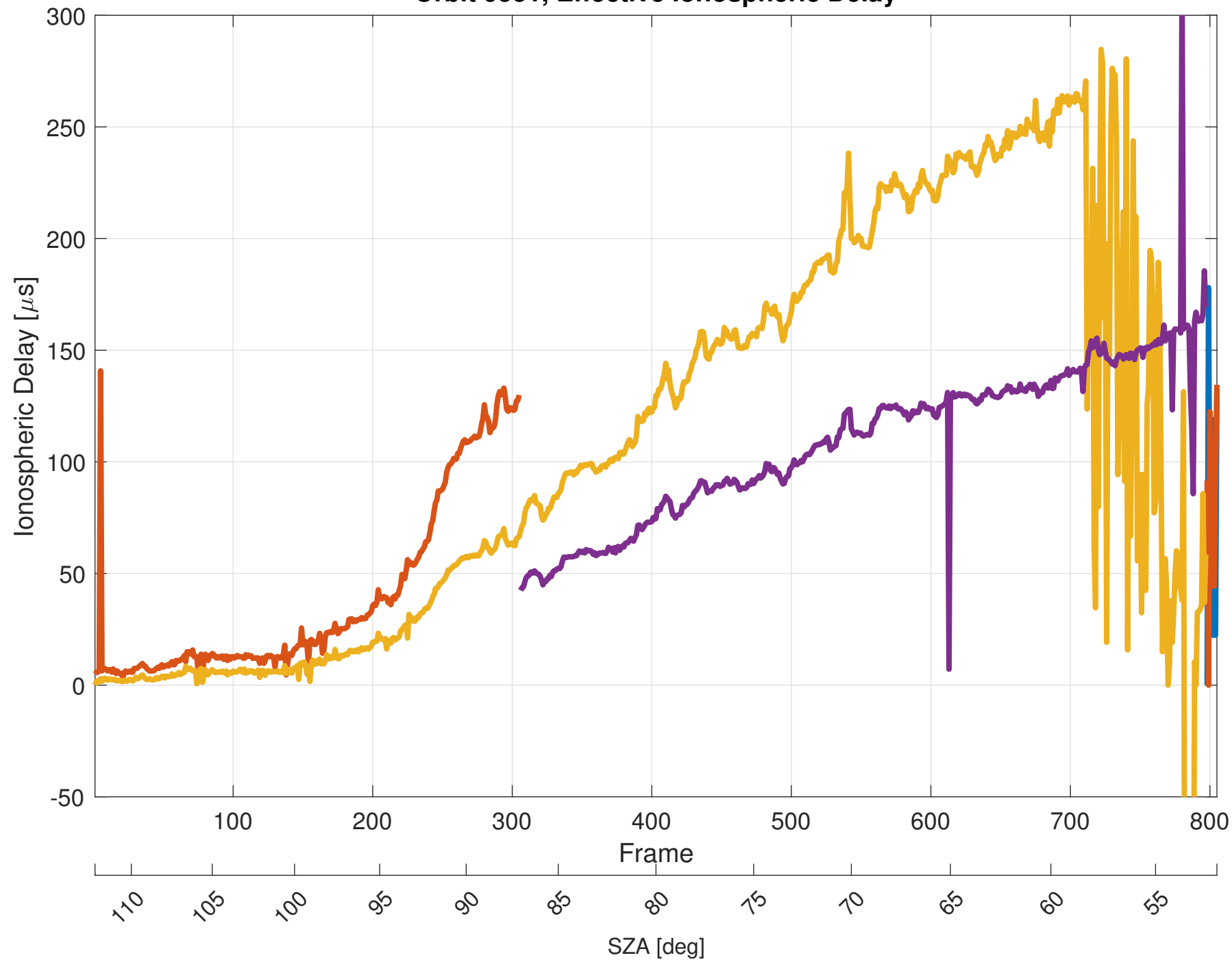
Orbit 9551, Effective Ionospheric Delay
