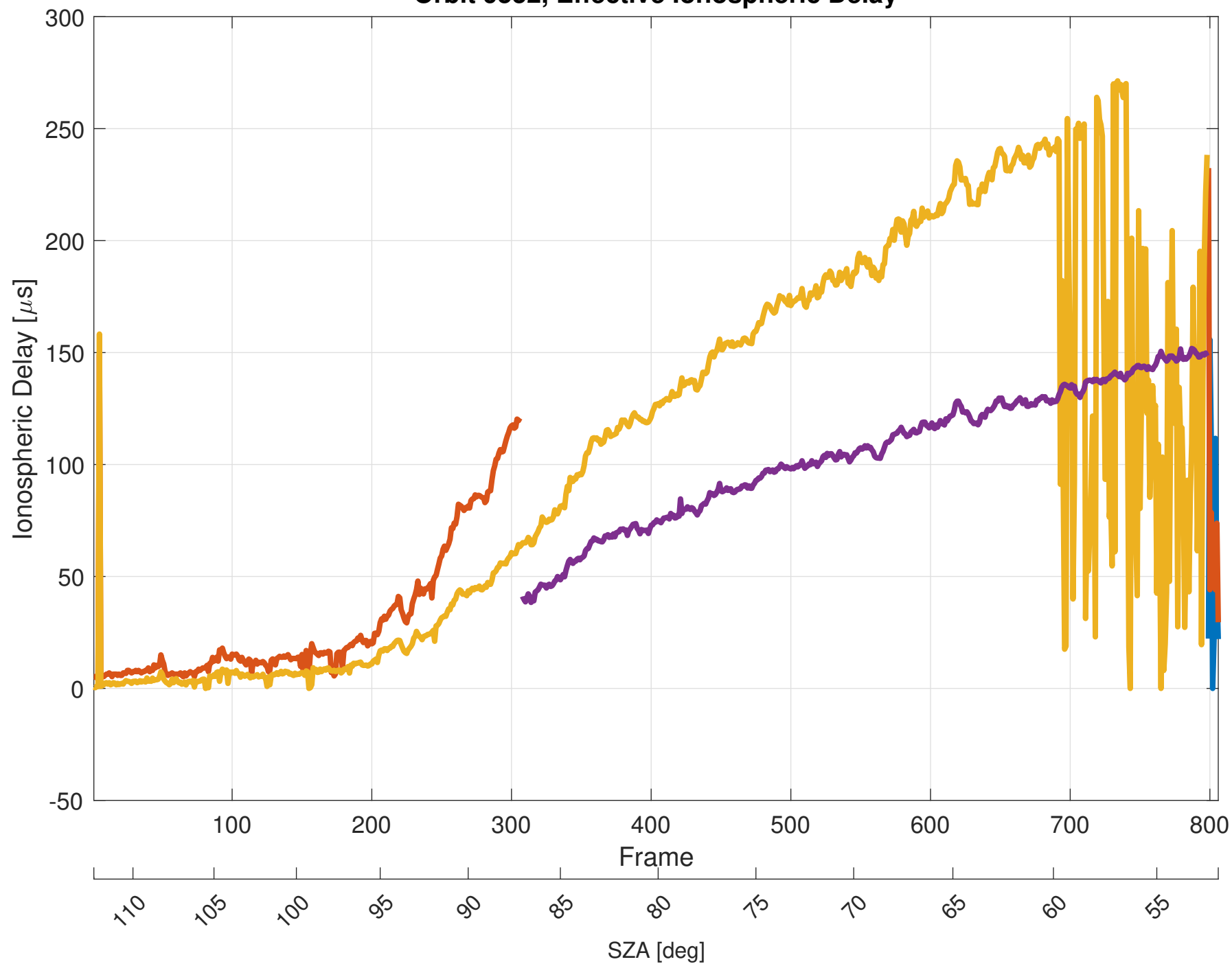
Orbit 9552, Effective Ionospheric Delay
