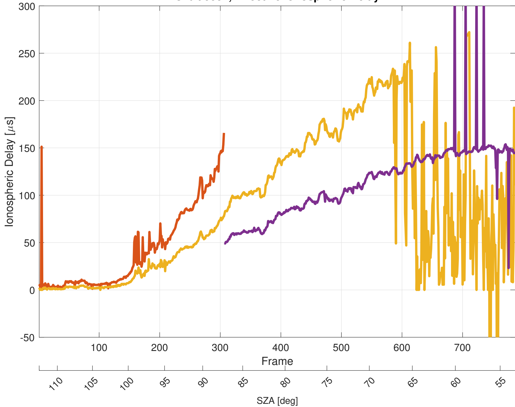
Orbit 9554, Effective Ionospheric Delay
