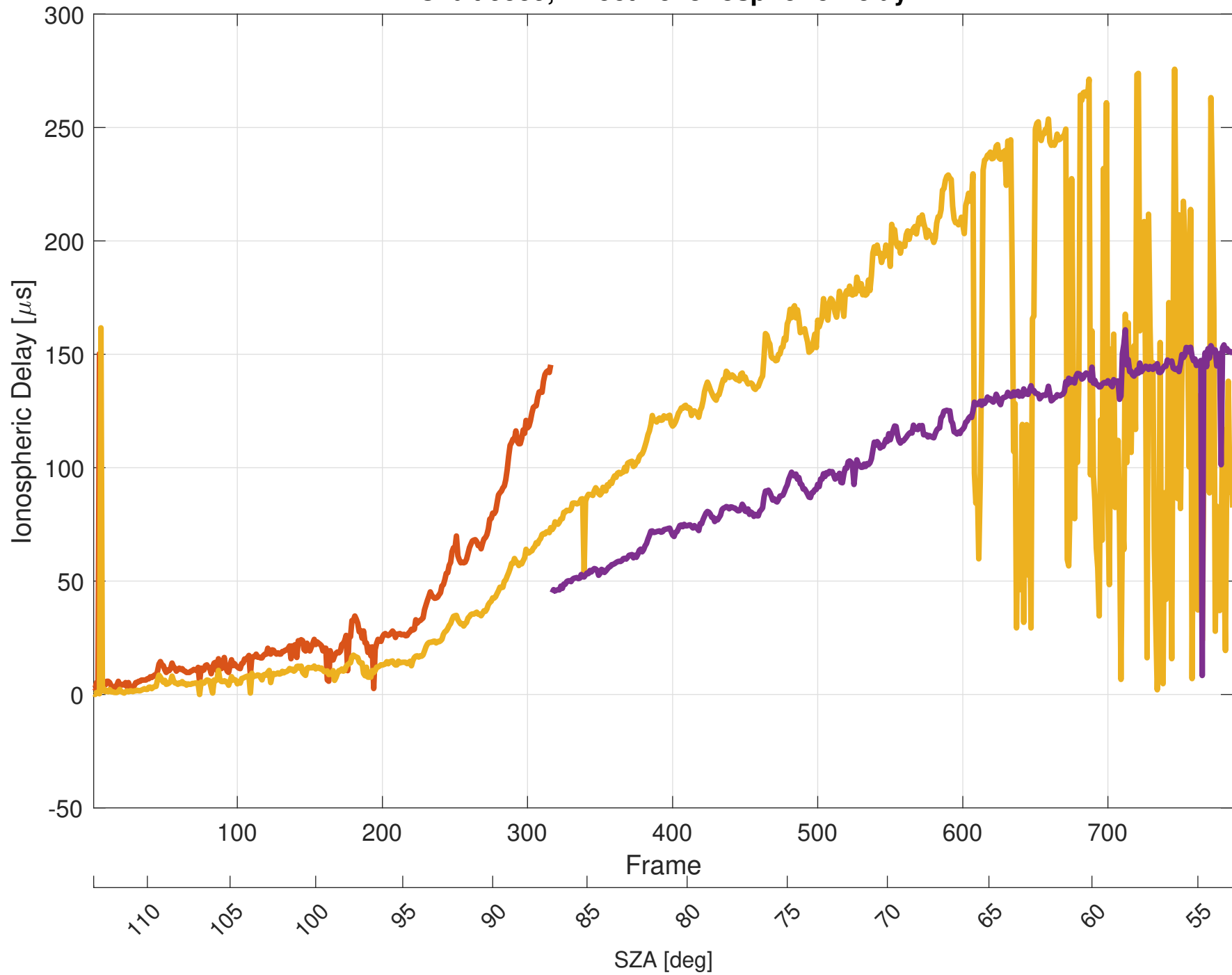
Orbit 9559, Effective Ionospheric Delay
