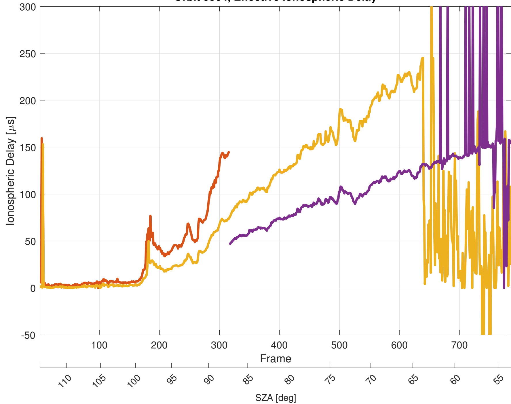
Orbit 9564, Effective Ionospheric Delay
