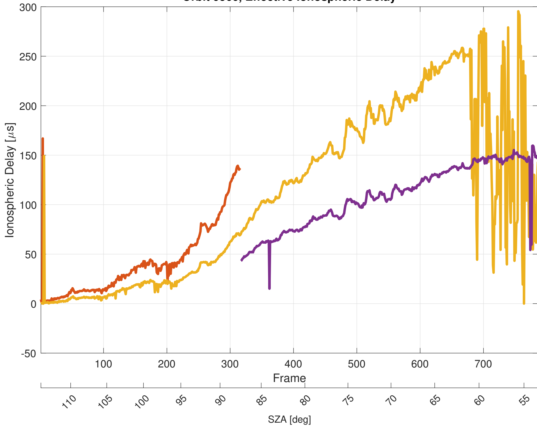
Orbit 9566, Effective Ionospheric Delay
