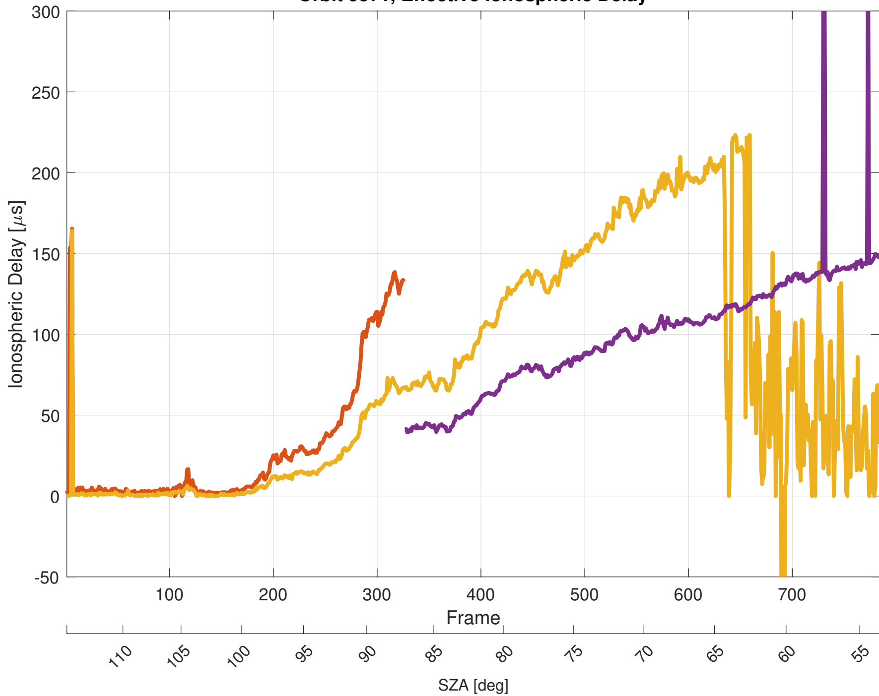
Orbit 9571, Effective Ionospheric Delay
